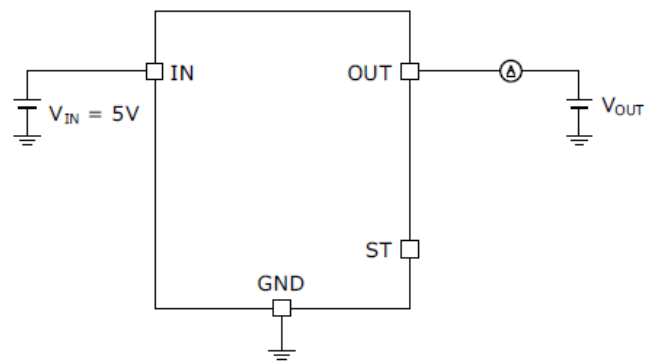
Measurement Circuit for Figure 18 and Figure 19
