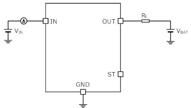
Measurement Circuit for Figure 3 and Figure 4
