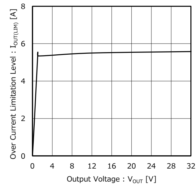
Figure 18. Over Current Limitation Level vs Output Voltage
