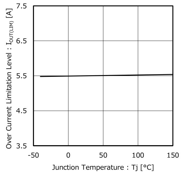
Figure 19. Over Current Limitation Level vs Junction Temperature (V OUT = 12 V, 24 V)
