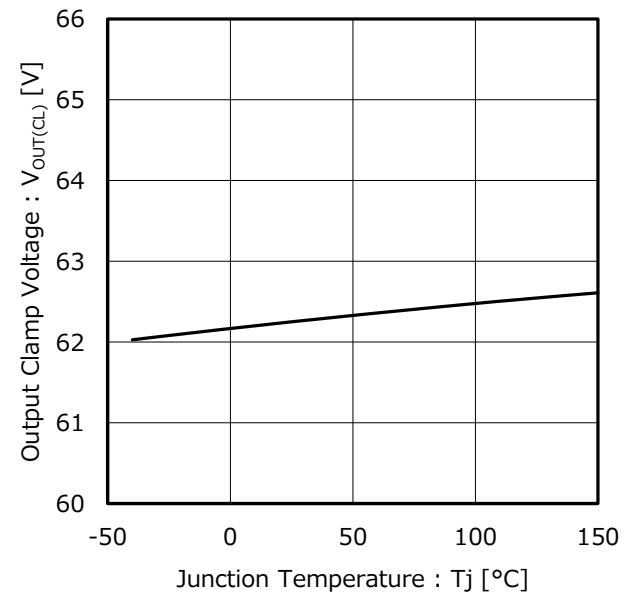
Figure 9. Output Clamp Voltage vs Junction Temperature (IOUT = 10 mA)
