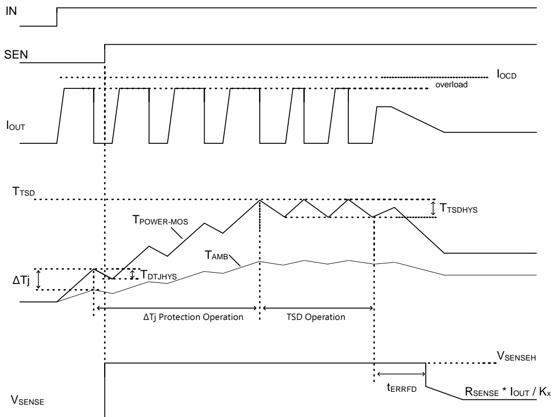
Figure 65. Overtemperature Protection
