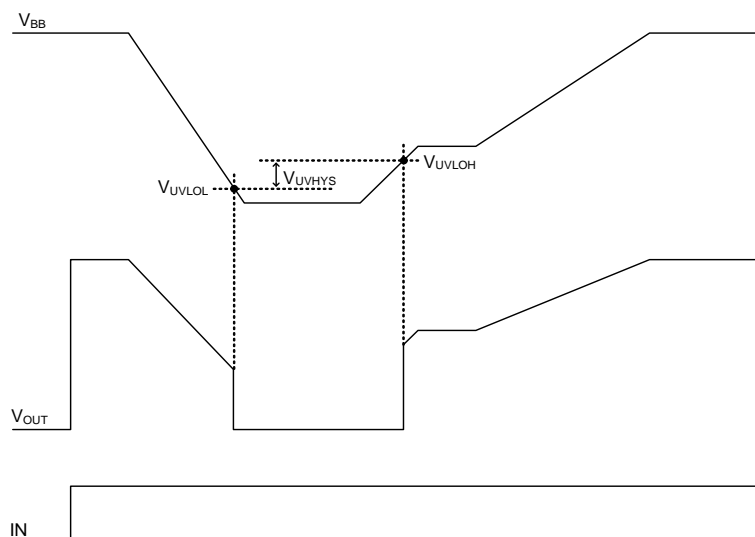
Figure 58. UVLO Functionality
