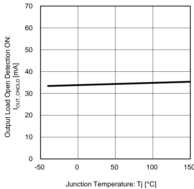
Figure 43. Output Load Open Detection ON vs Junction Temperature
