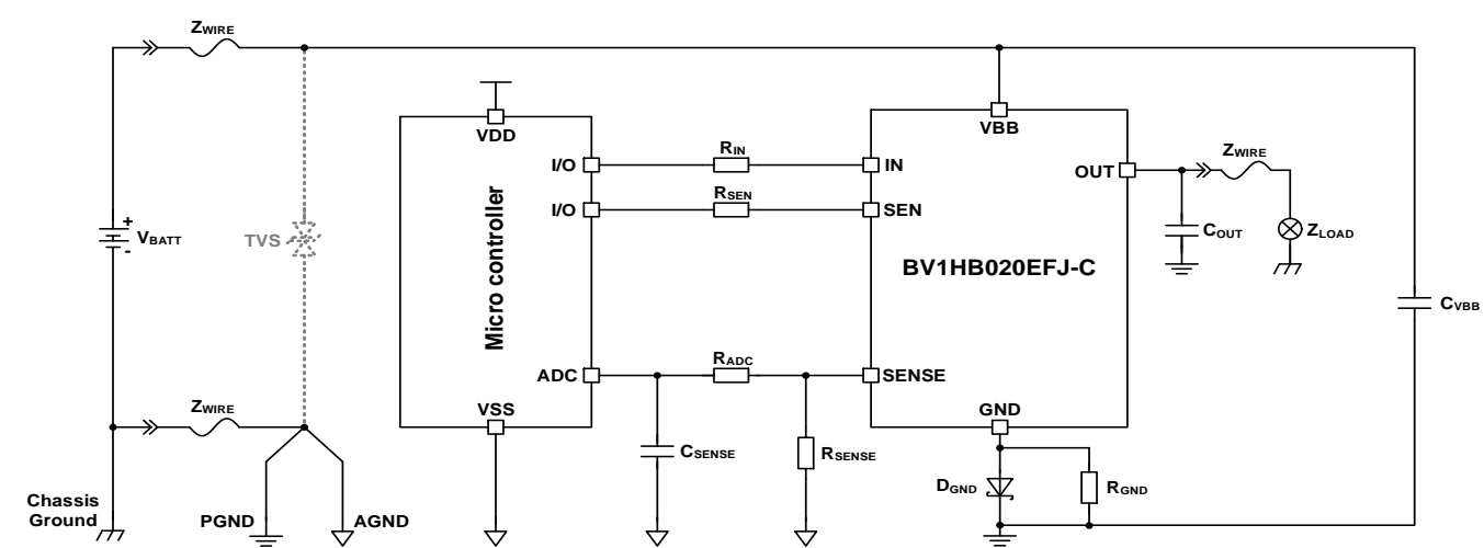
Figure 72. Application Schematic
