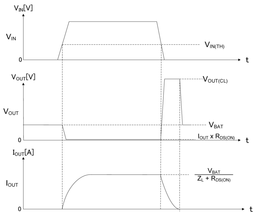
Figure 26. Inductive Load Operation
