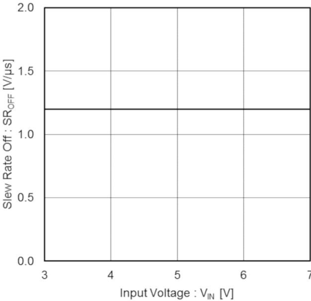
Figure 11. Slew Rate Off vs Input Voltage
