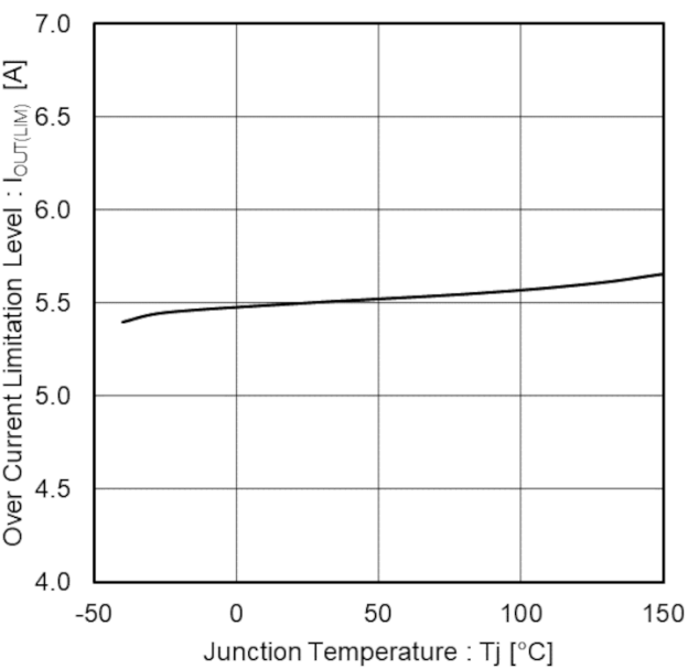
Figure 18. Over Current Limitation Level vs Junction Temperature
