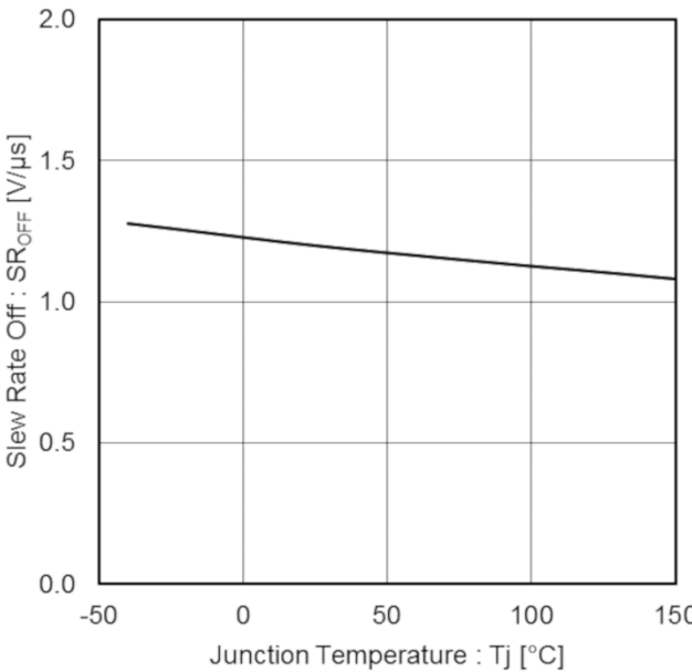
Figure 13. Slew Rate Off vs Junction Temperature
