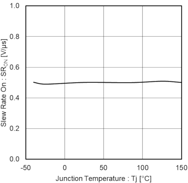
Figure 12. Slew Rate On vs Junction Temperature
