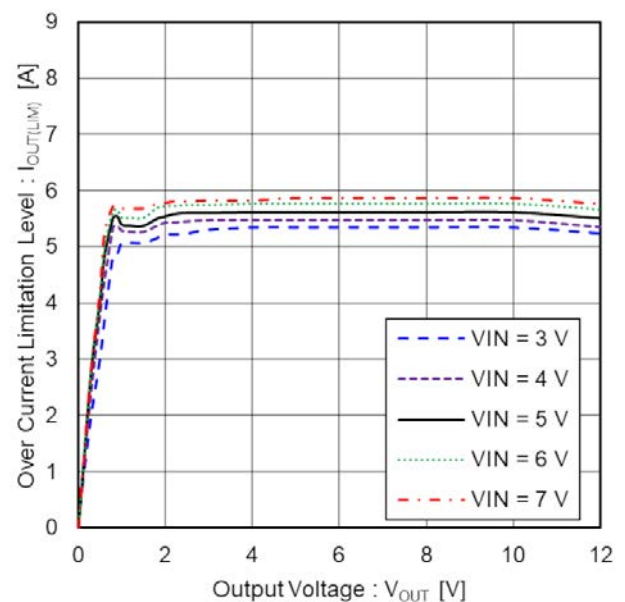
Figure 17. Over Current Limitation Level vs Output Voltage
