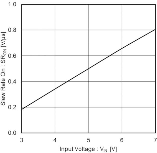
Figure 10. Slew Rate On vs Input Voltage
