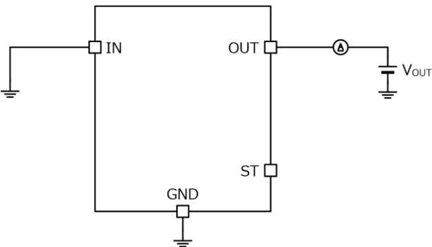
Measurement Circuit for Figure 5
