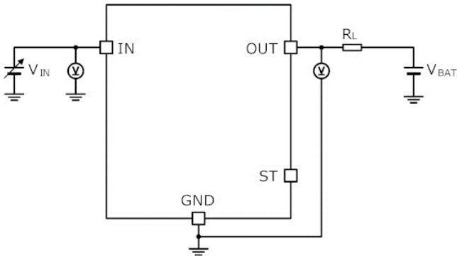
Measurement Circuit for Figure 2
