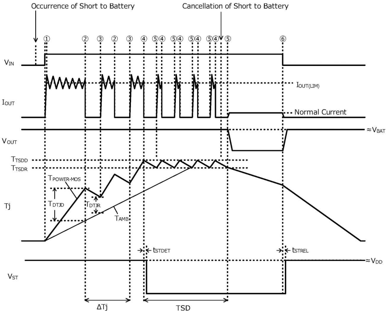
Figure 23. The Behavior When OUT Pin is shorted to Battery
