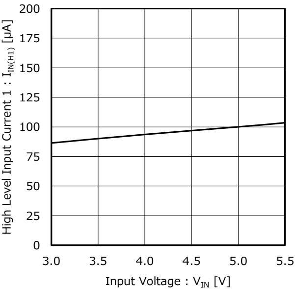
Figure 3. High Level Input Current 1 vs Input Voltage
