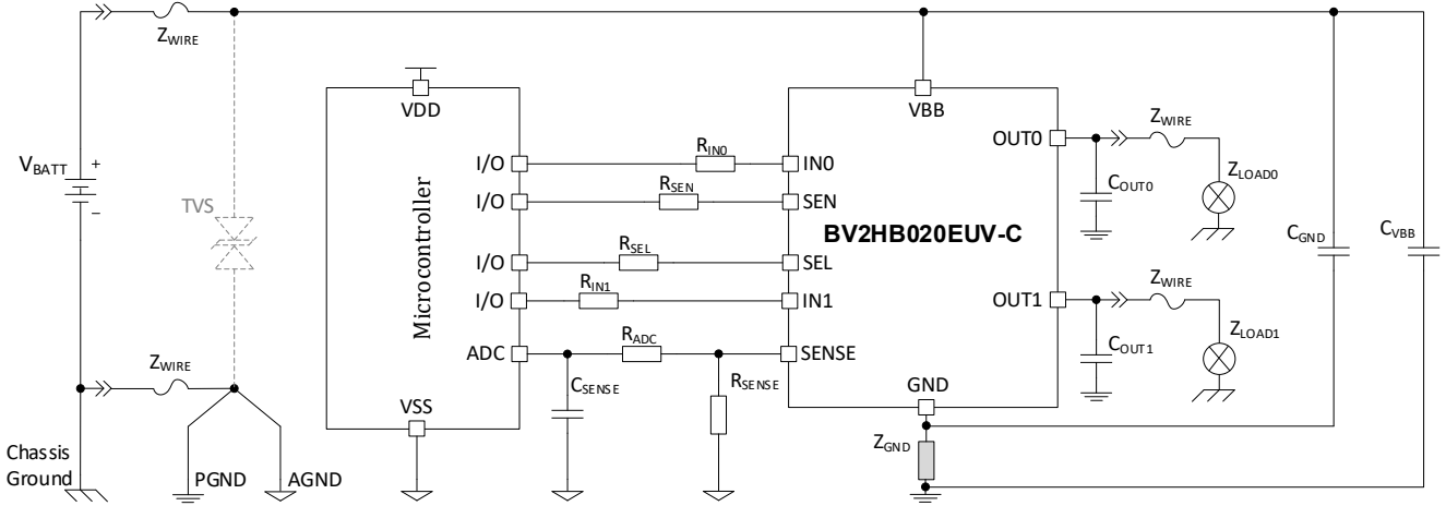
Figure 74. Application Schematic
