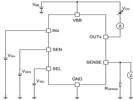
Figure 53. Open Load at OFF V_{DS} Detect Diagnostic Error Flag Voltage
