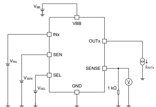
Figure 57. Current Sense Ratio
