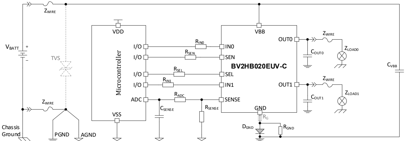
Figure 76. Application Schematic Example – Semiconductor Diode Ground Protection Network k
