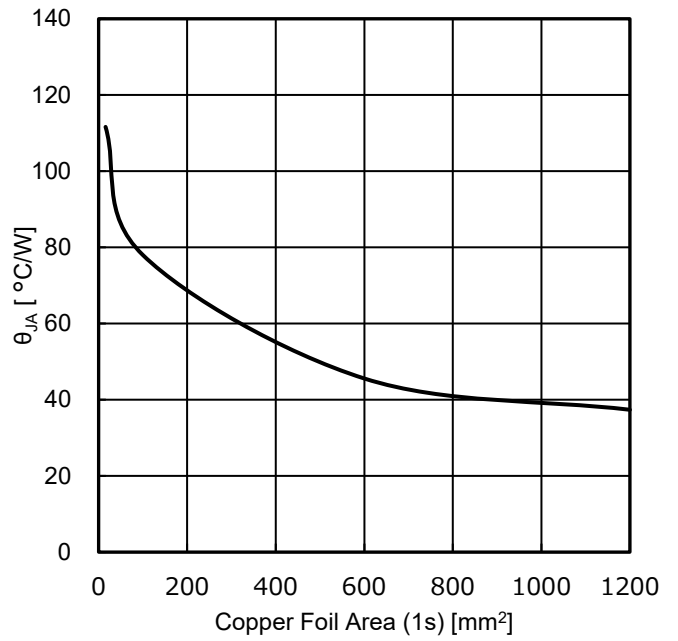
Figure 9. Thermal Resistance (One Output-Channel Active)
