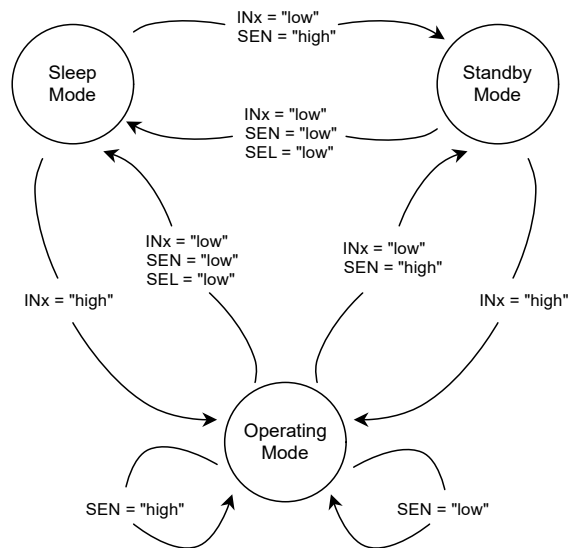
Figure 59. State Diagram
