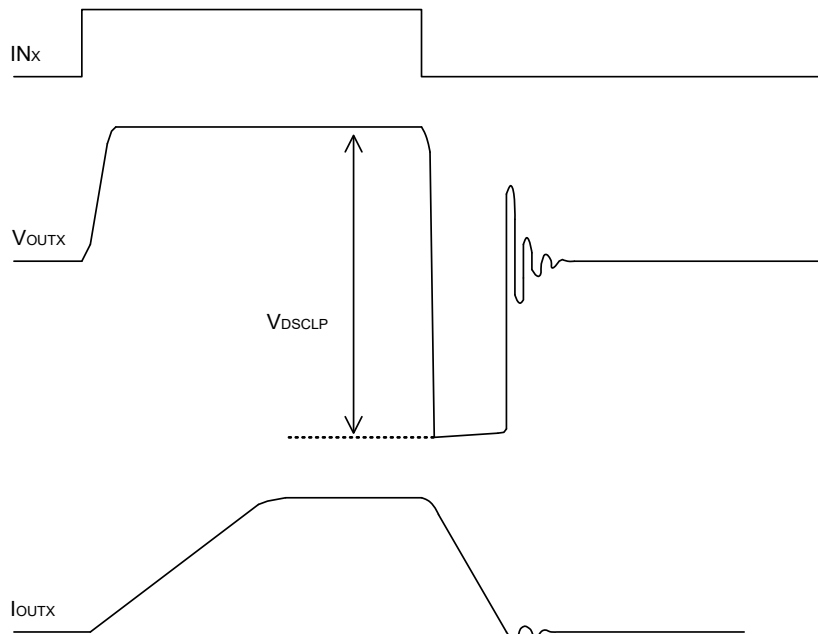
Figure 62. Switching Inductive Loads
