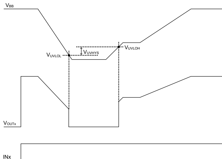
Figure 60. UVLO Functionality
