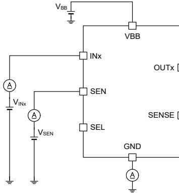
Figure 47. Standby Mode Current Operating Mode Current
