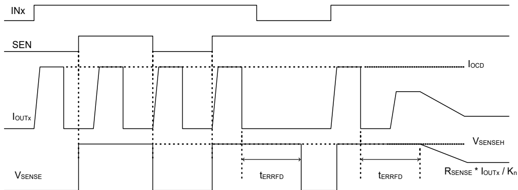
Figure 68. Overcurrent Protection
