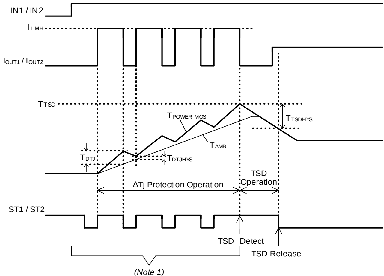
Figure 39. Thermal Shutdown Protection and \Delta T_j Protection Timing Chart
