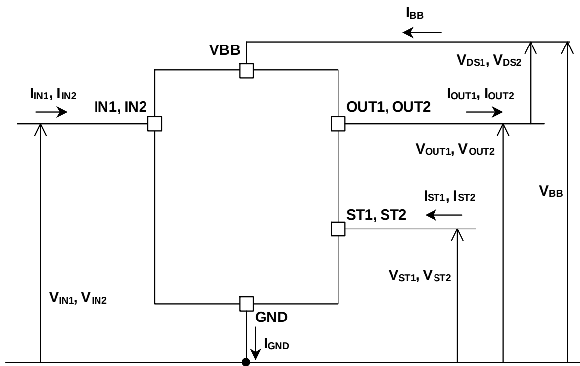
Figure 4. Voltage and Current Definition
