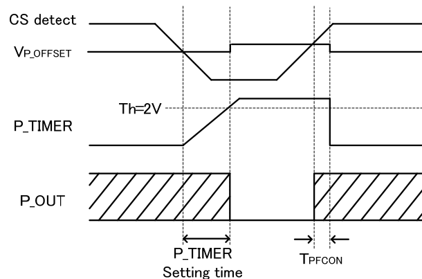
Figure 40. Timing Chart
