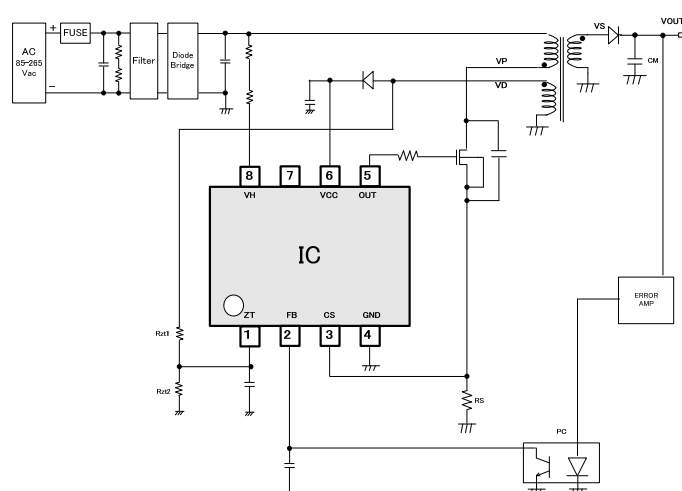
Figure 1. Application Circuit
