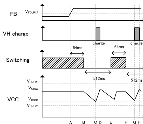
Fg-25 Over Load Protection : Auto-recovery
