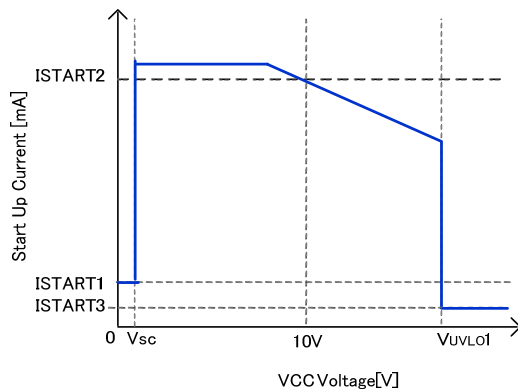
Figure-6 Start-up Current vs VCC Voltage
