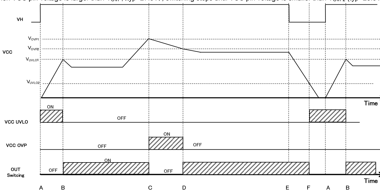
Figure-11 VCC UVLO / OVP Timing Chart
