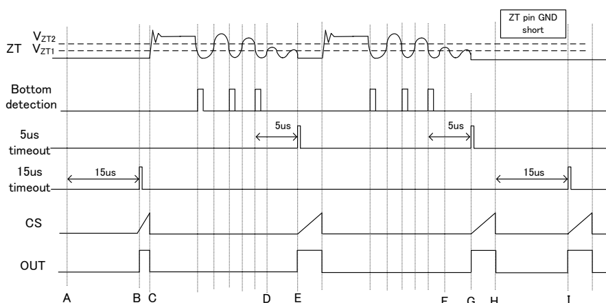
Figure-22 ZT Timeout Function
