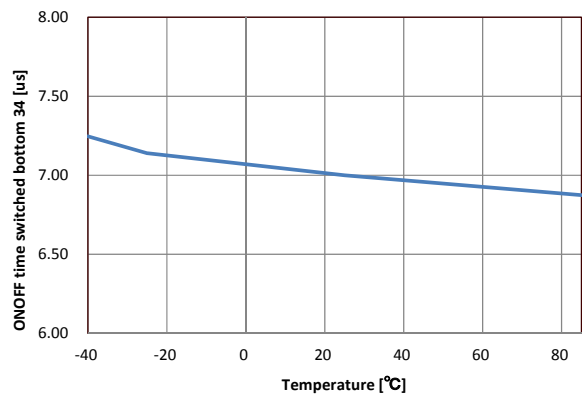
Figure 42 ONOFF time switched bottom 34 vs Temperature
