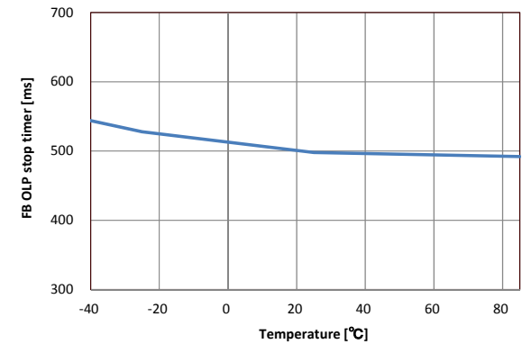
Figure 51 FBOLP stop timer vs Temperature
