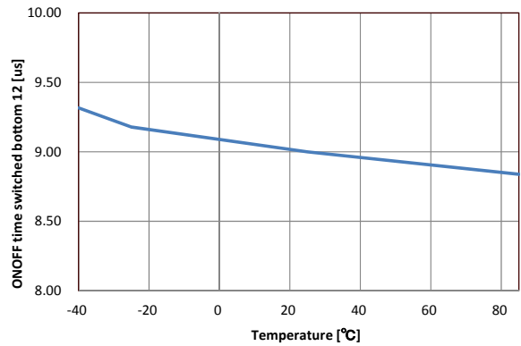
Figure 40 ONOFF time switched bottom 12 vs Temperature
