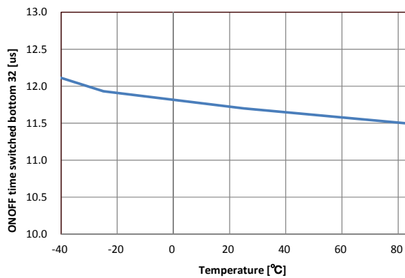
Figure 45 ONOFF time switched bottom 32 vs Temperature
