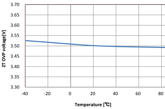
Figure 49 ZT OVP voltage vs Temperature
