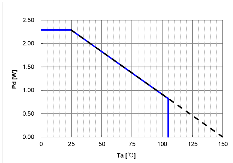
Figure 15. Thermal Abatement Characteristic
