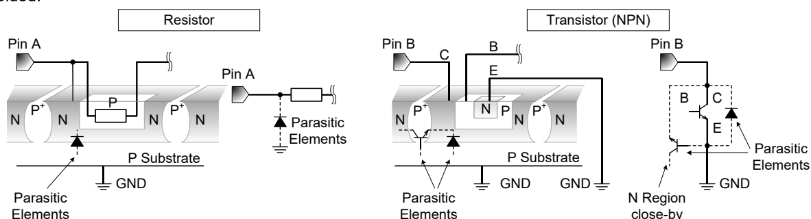
Figure 29. Example of IC Structure
