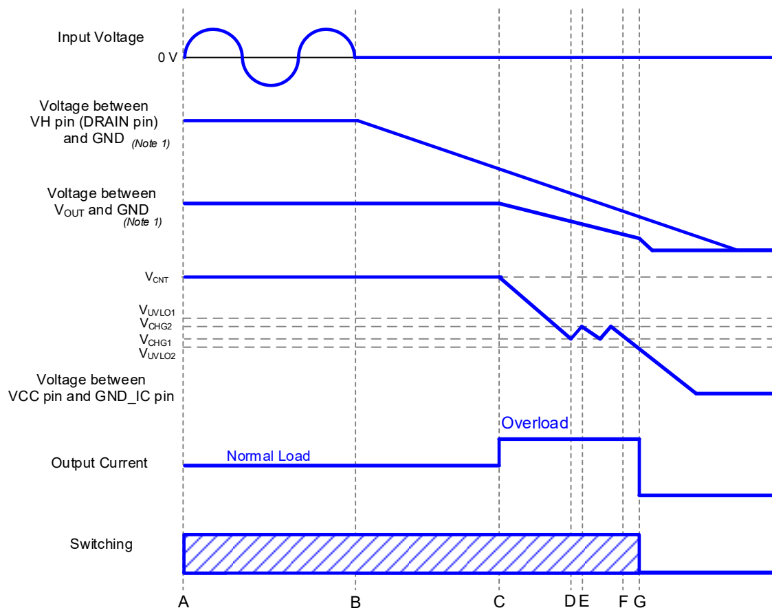
Figure 4. Stop Sequences Timing Chart
