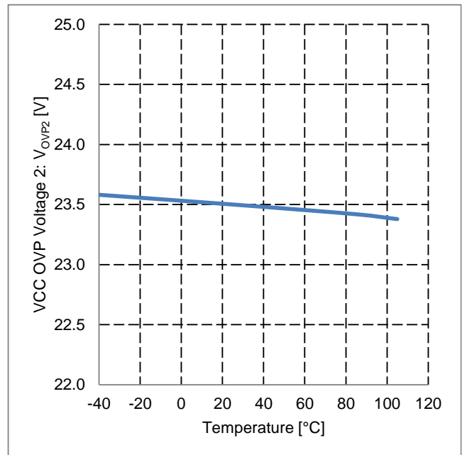
Figure 22. VCC OVP Voltage 2 vs Temperature
