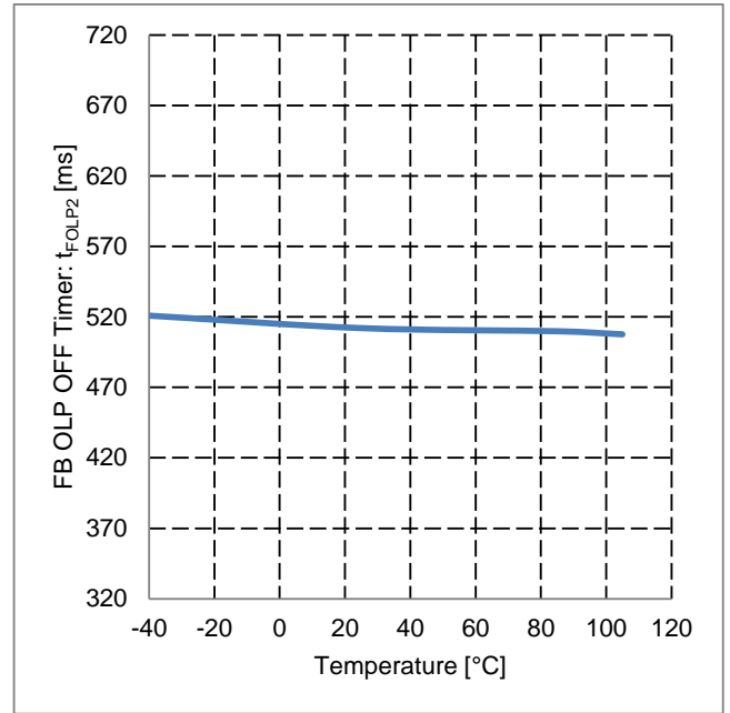
Figure 40. FB OLP OFF Timer vs Temperature
