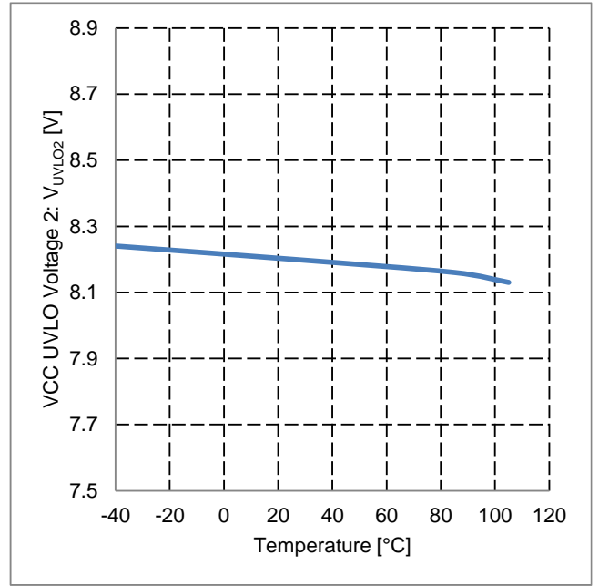
Figure 20. VCC UVLO Voltage 2 vs Temperature
