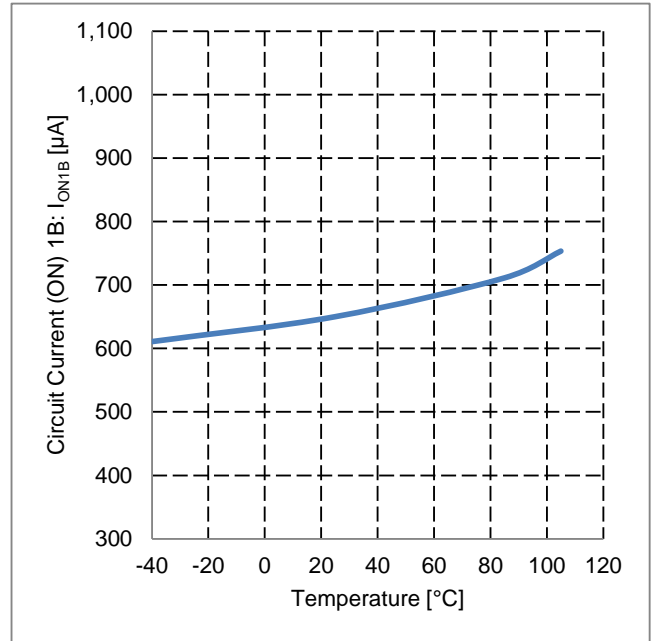
Figure 16. Circuit Current (ON) 1B vs Temperature
