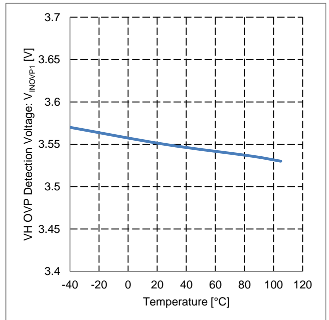
Figure 46. VH OVP Detection Voltage vs Temperature
