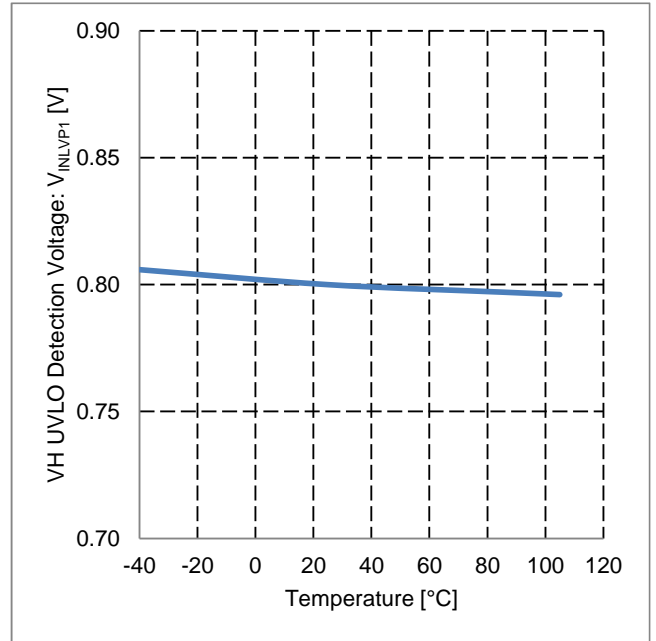
Figure 44. VH UVLO Detection Voltage vs Temperature
