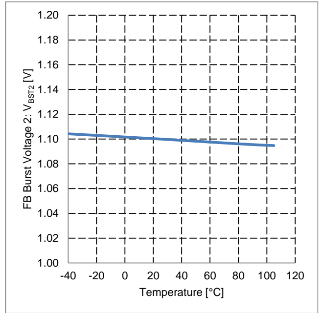
Figure 32. FB Burst Voltage 2 vs Temperature
