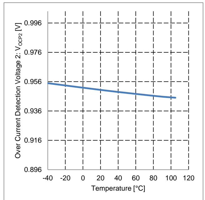
Figure 42. Over Current Detection Voltage 2 vs Temperature
