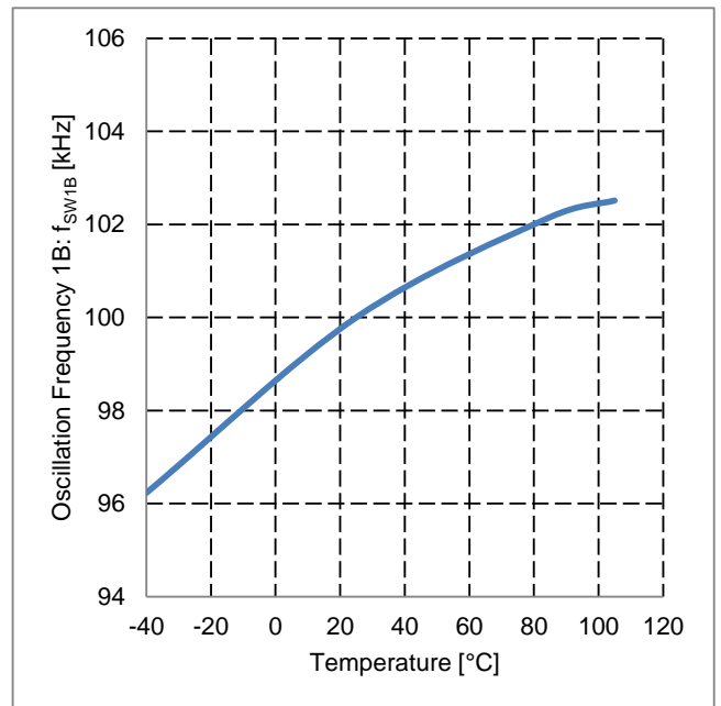
Figure 26. Oscillation Frequency 1B vs Temperature
