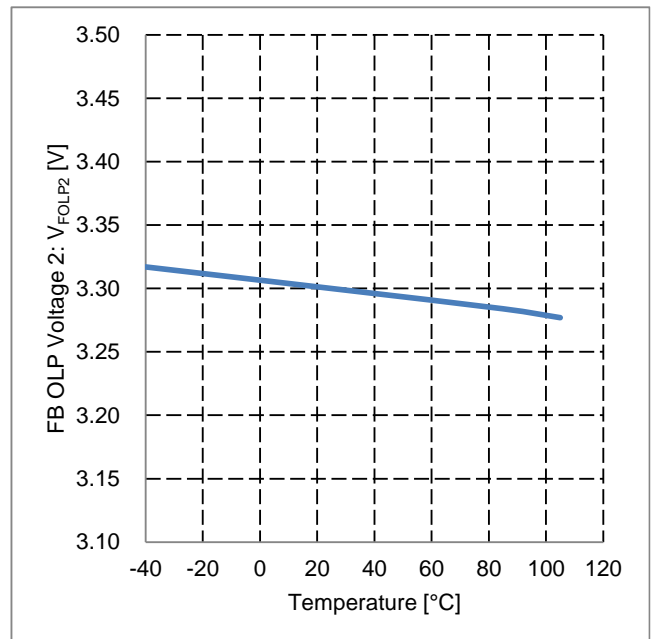
Figure 38. FB OLP Voltage 2 vs Temperature
