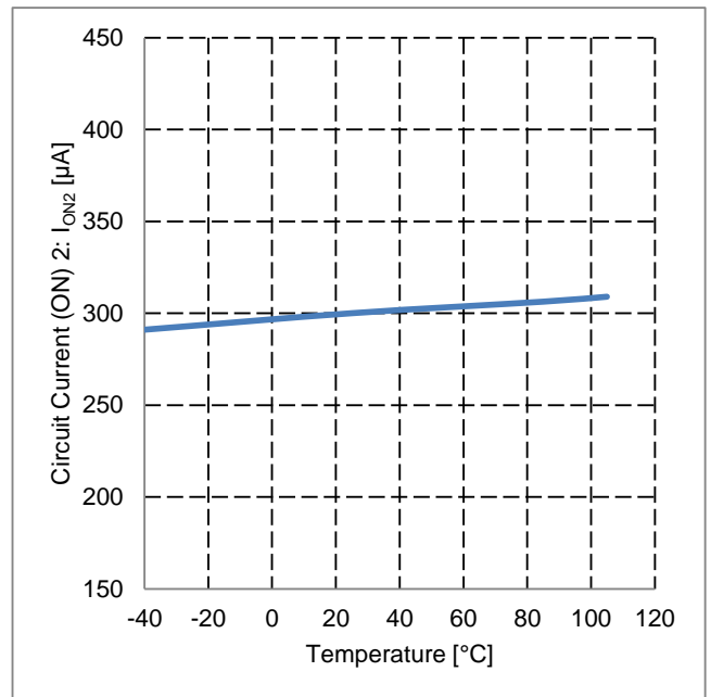
Figure 18. Circuit Current (ON) 2 vs Temperature
