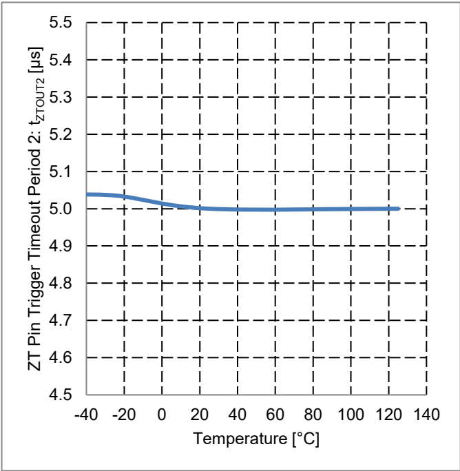
Figure 43. ZT Pin Trigger Timeout Period 2 vs Temperature
