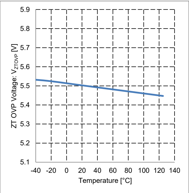
Figure 50. ZT OVP Voltage vs Temperature
