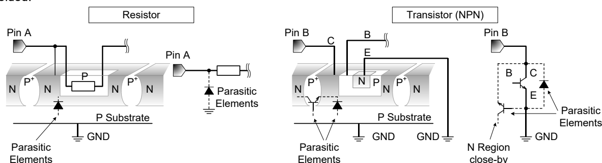
Figure 56. Example of IC Structure
