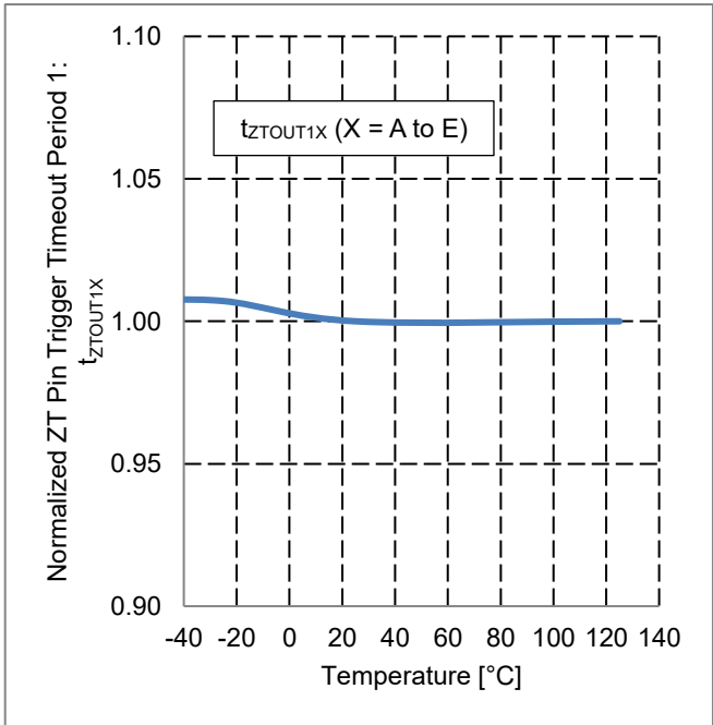
Figure 42. Normalized ZT Pin Trigger Mask Timeout Period 1 vs Temperature
