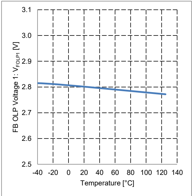
Figure 46. FB OLP Voltage 1 vs Temperature
