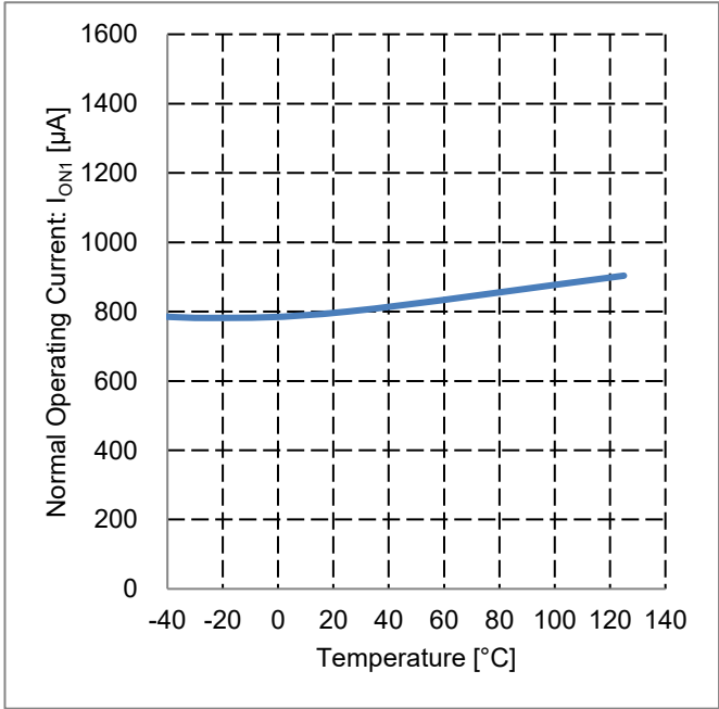
Figure 21. Normal Operating Current vs Temperature
