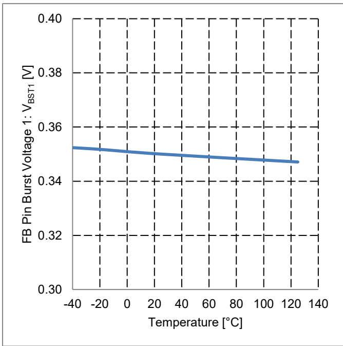
Figure 35. FB Pin Burst Voltage 1 vs Temperature
