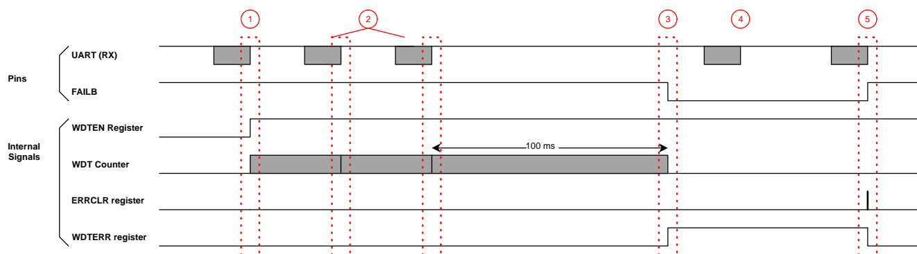
Figure 68. WDT Protection
