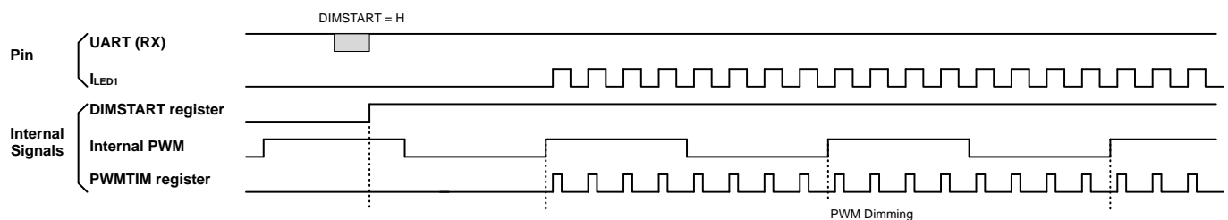
Figure 51. PWMFREQ = 3
