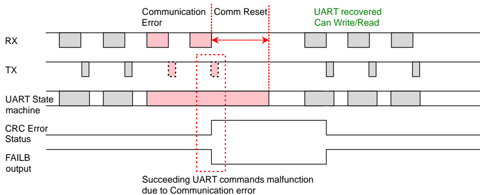
Figure 28. Communication Reset
