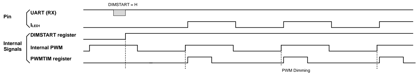
Figure 48. PWMFREQ = 0
