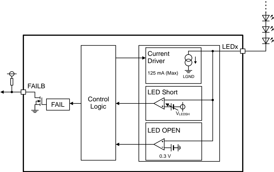
Figure 41. LED Pin Protection Circuit Image
