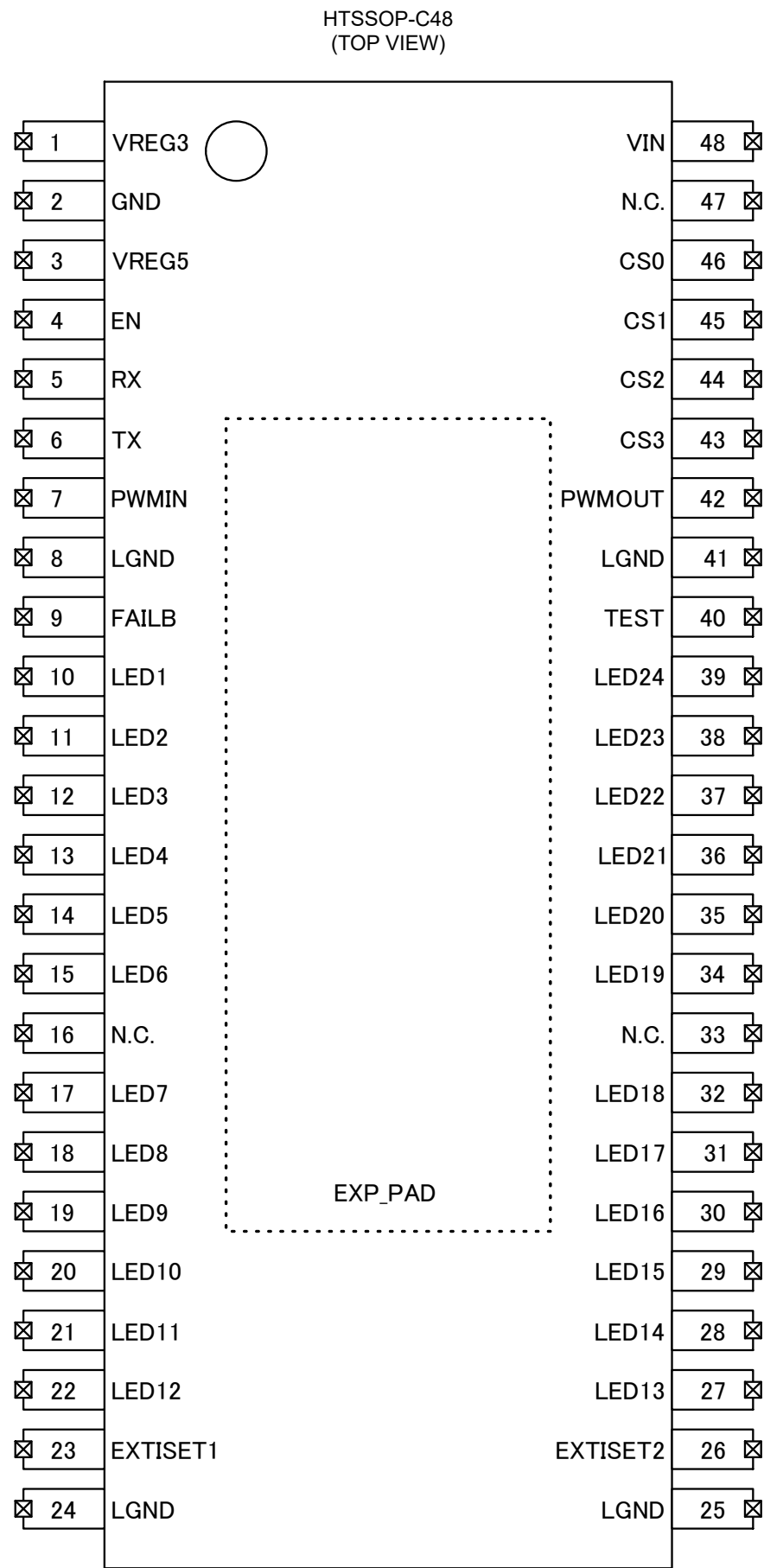
Figure 2. Pin Configuration
