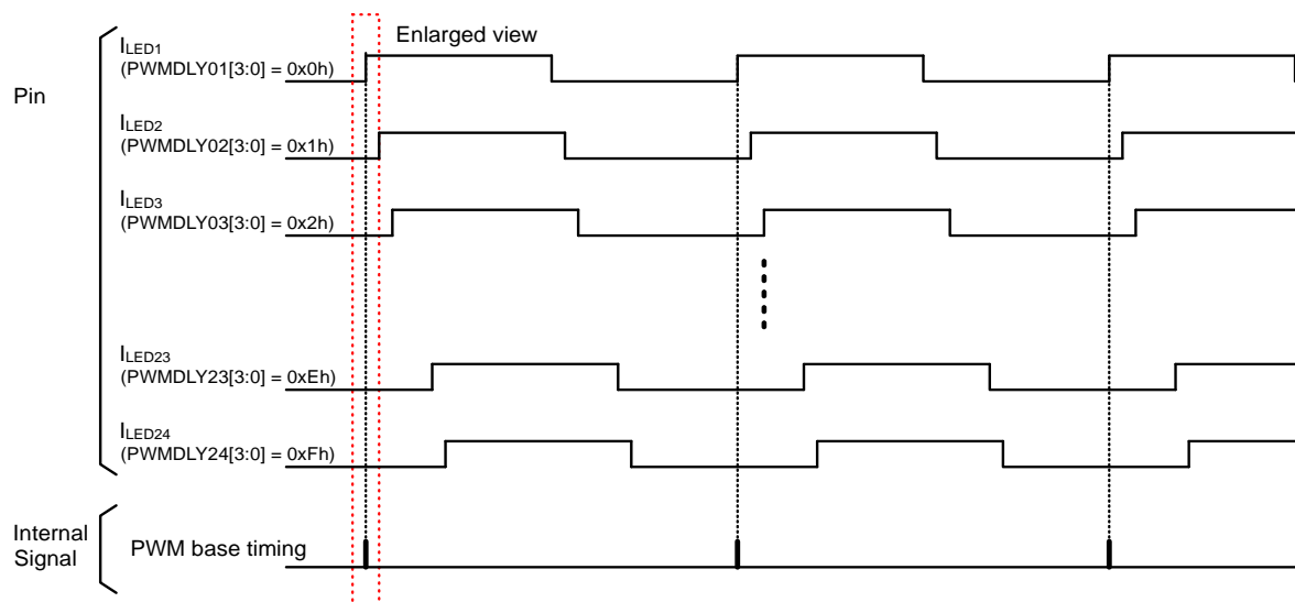
Figure 42. PWM Delay Setting
