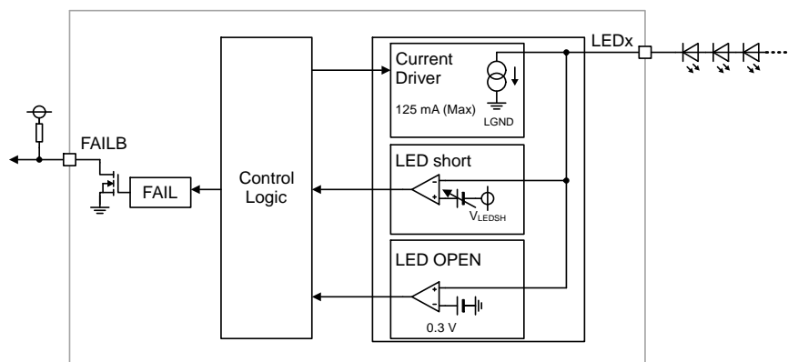
Figure 6. LED Open Detection
