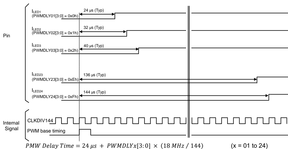
Figure 43. PWM Delay Setting (Enlarged View)
