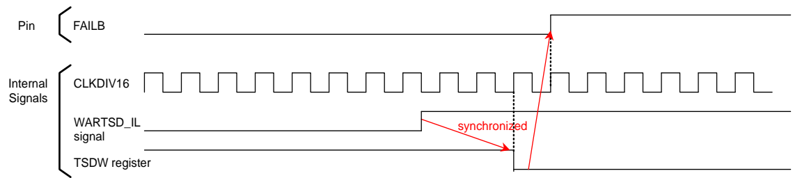
Figure 57. TSD Warning Released Function (Enlarged View B)
