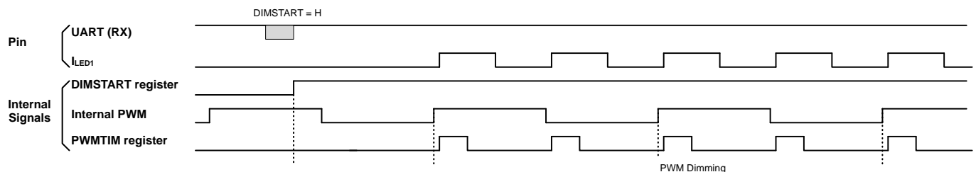
Figure 49. PWMFREQ = 1
