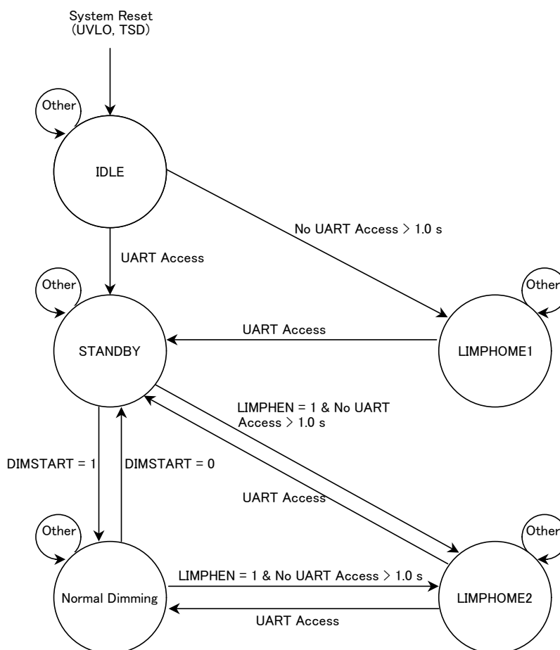
Figure 9. LIMPHOME Function
