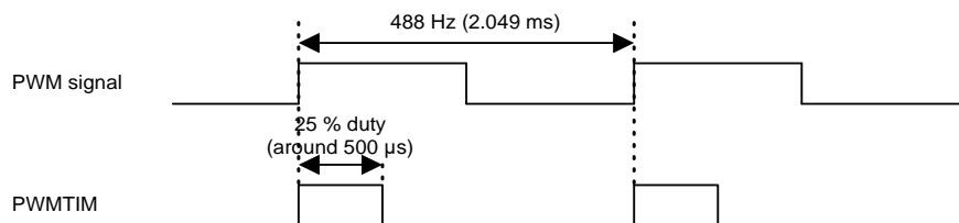
Figure 32. PWMTIM Image
