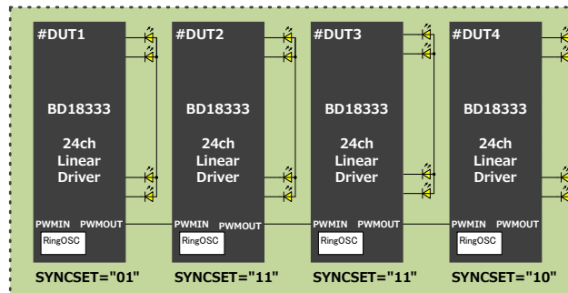
Figure 40. SYNCSET setting for multiple connection
