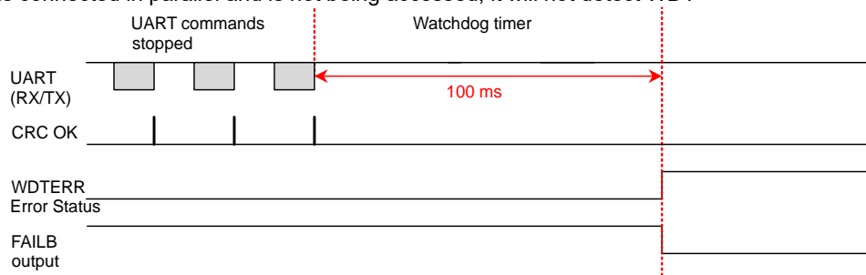
Figure 29. Watchdog Timer
