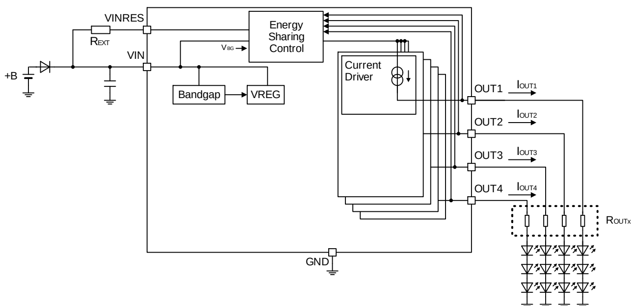
Figure 8. Energy Sharing Control
