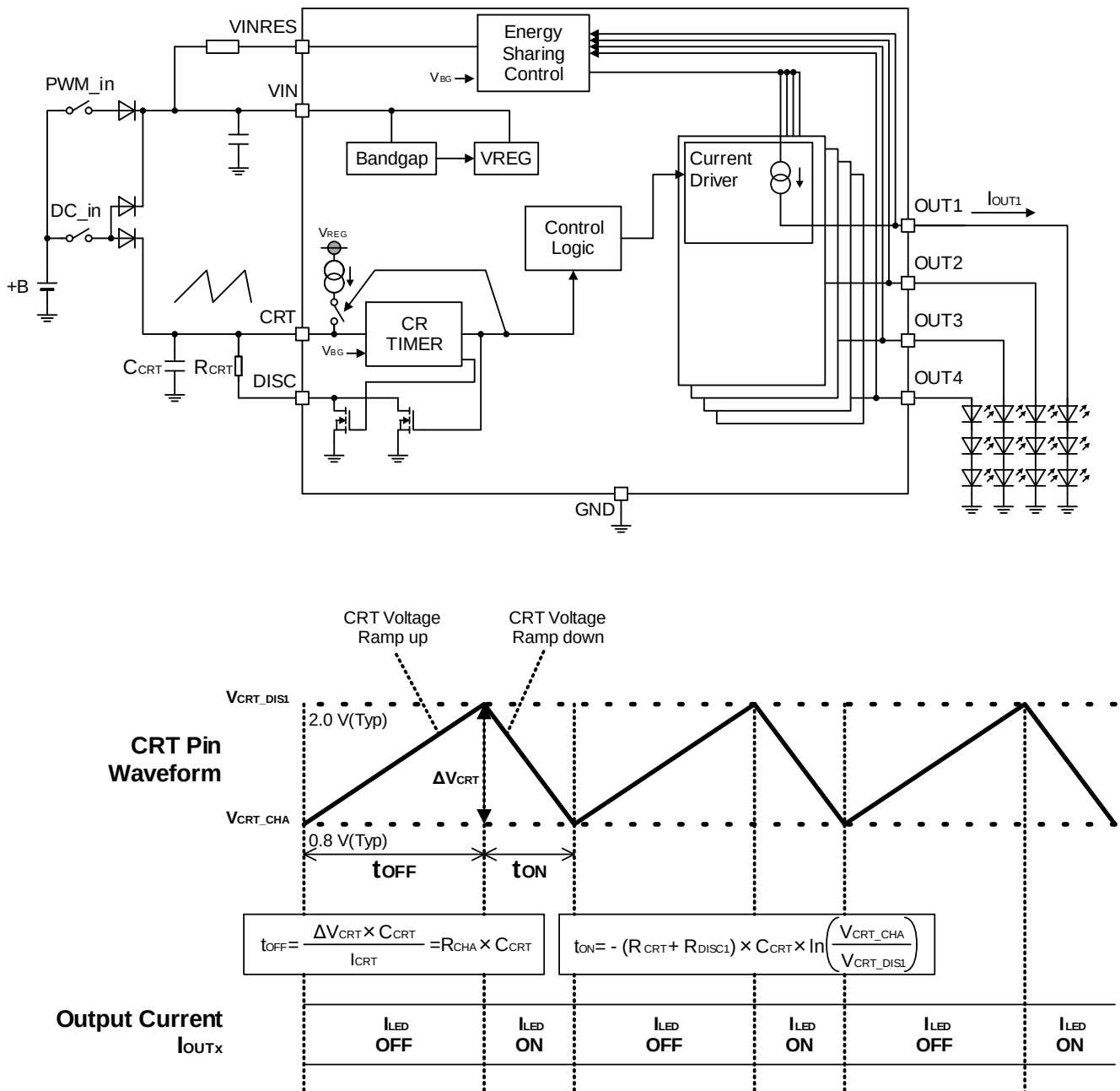
Figure 12. PWM Dimming Operation
