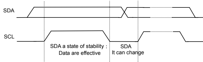
Figure 3. Bit Transfer
