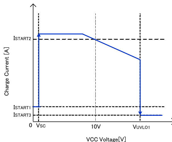
Figure 6. Charge Current—VCC Voltage Curve
