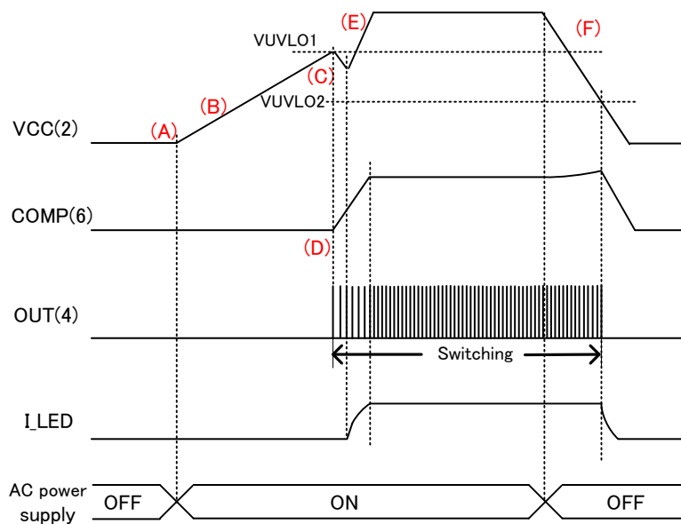
Figure 8. ON/OFF Sequences
