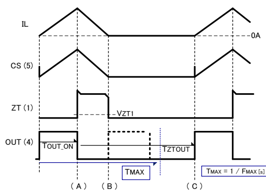
Figure 13. Maximum Frequency Operation
