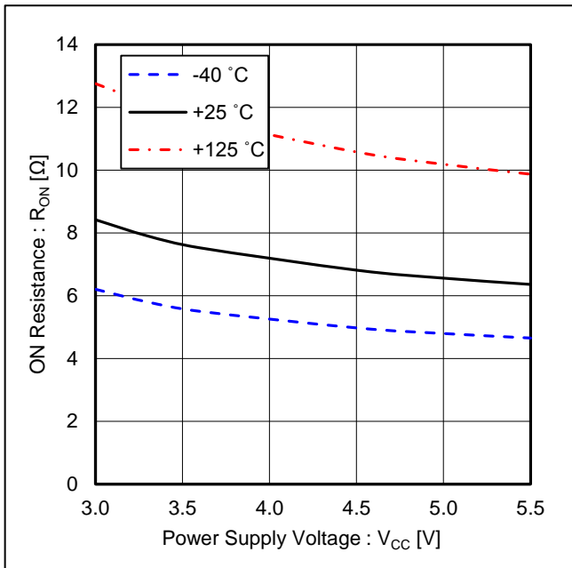
Figure 7. ON Resistance vs Power Supply Voltage (@ I_{DN} = 20 \text{ mA} )
