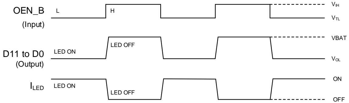
Figure 2. PWM Dimming Control
