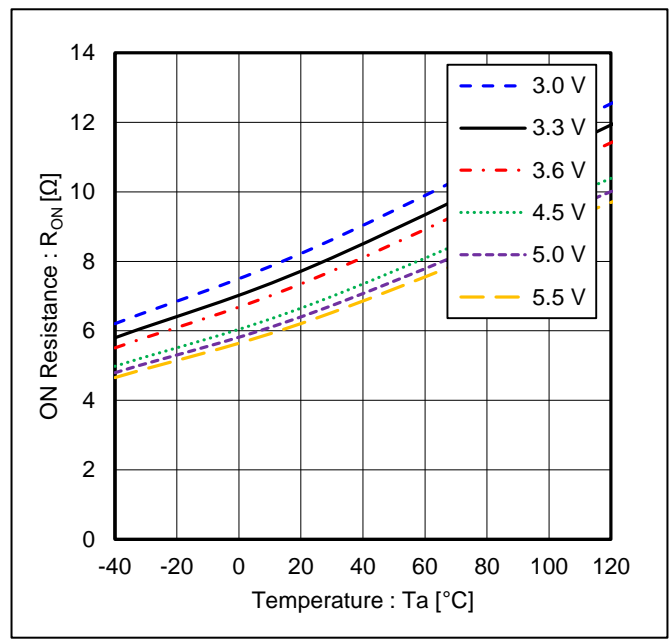
Figure 8. ON Resistance vs Temperature (@ I_{DN} = 20 \text{ mA} )
