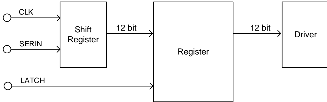
Figure 1. Block Diagram of Serial Communication
