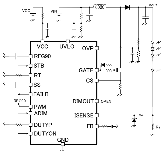
Figure 15. Example circuit for analog dimming
