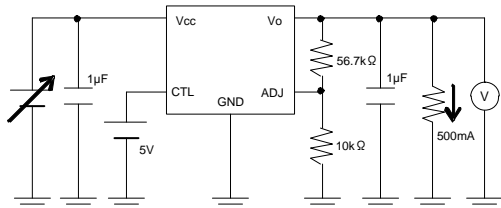
Measurement Circuit of Figure 7
