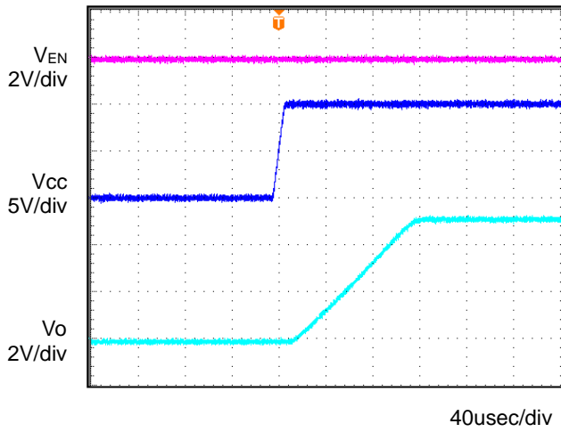
Figure 2. Input sequence ( C_{OUT} = 1\mu\text{F} )
