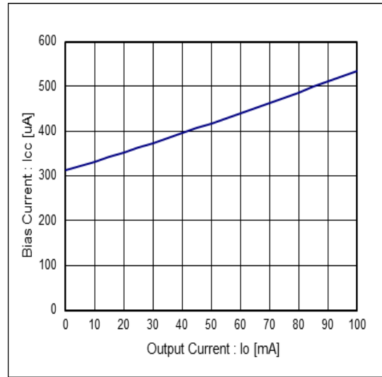
Figure 11. I_{CC} - I_O
