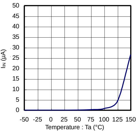
Figure 21. I INSTB VS Temperature
