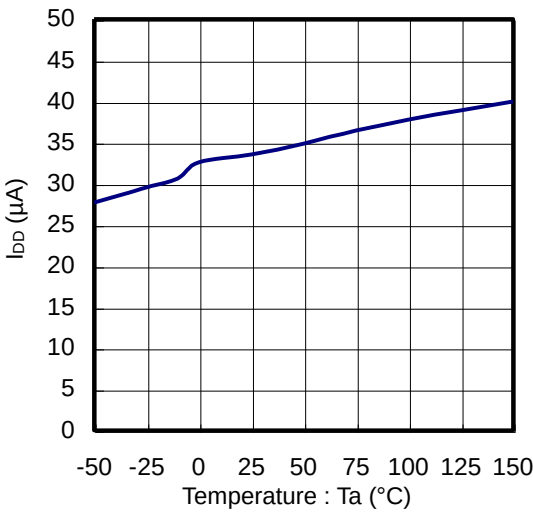
Figure 18. I DD vs Temperature
