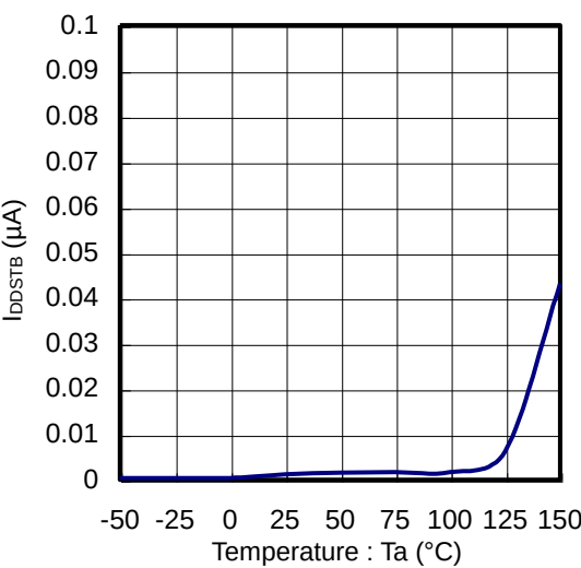
Figure 19. I DDSTB VS Temperature
