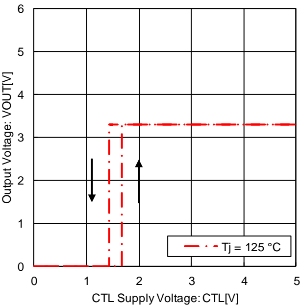
Figure 20. CTL ON / OFF Mode Voltage (Tj = 125 °C)
