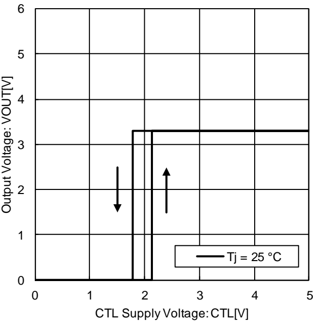
Figure 19. CTL ON / OFF Mode Voltage (Tj = 25 °C)
