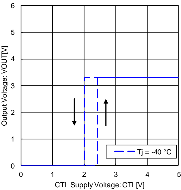
Figure 18. CTL ON / OFF Mode Voltage (Tj = -40 °C)
