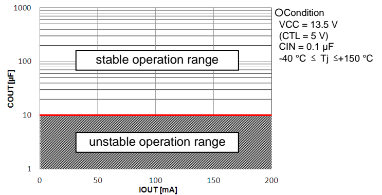
Figure 42. COUT (Typ.) vs. IOUT
