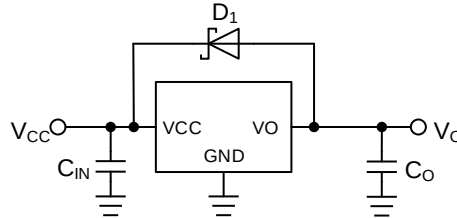
Figure 13. Bypass Diode for Reverse Current Diversion
