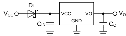
Figure 16. Protection against Reverse Polarity 1
