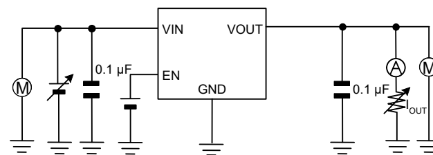
Measurement Setup for Figure 19 to 26, 41 to 48
