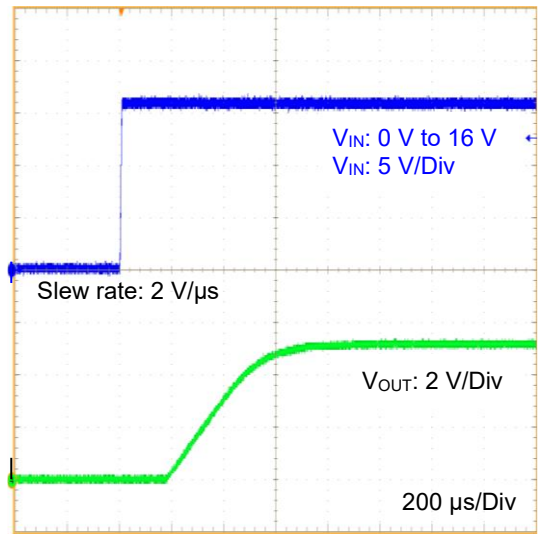
Figure 28. VIN Startup Waveform V_{IN}: 0\text{ V to }16\text{ V} (5 V output, I_{OUT} = 500\text{ mA} )
