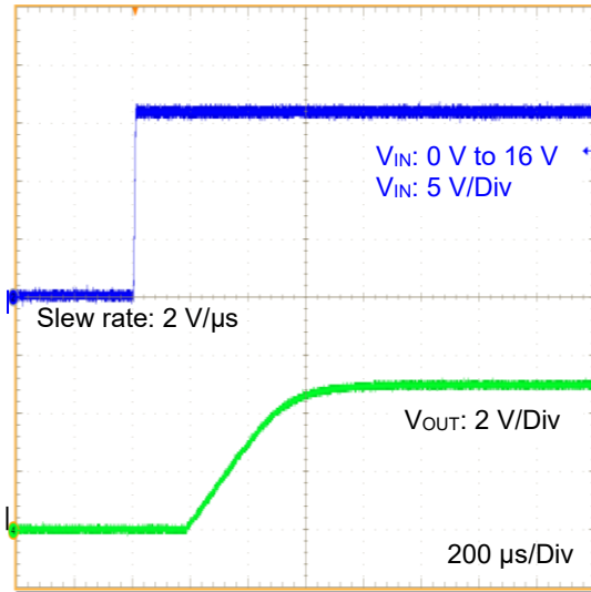
Figure 27. VIN Startup Waveform V_{IN}: 0\text{ V to }16\text{ V} (5 V output, I_{OUT} = 0\text{ mA} )
