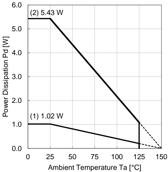
Figure 67. Power Dissipation Graph (TO252-3 / TO252-5)
