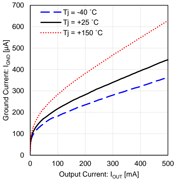
Figure 33. Ground Current vs Output Current (3.3 V output)
