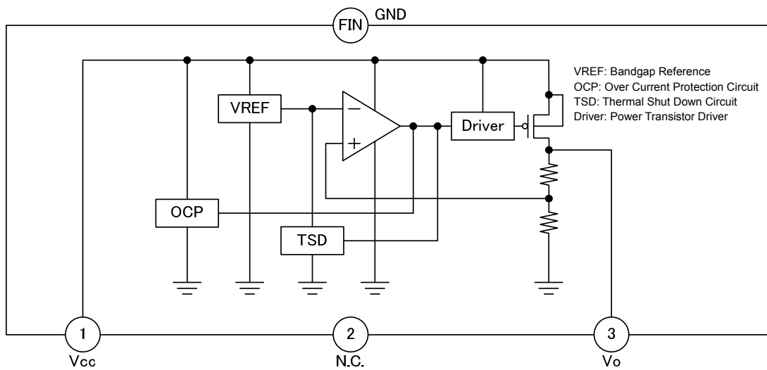
Figure 3. Block Diagram
