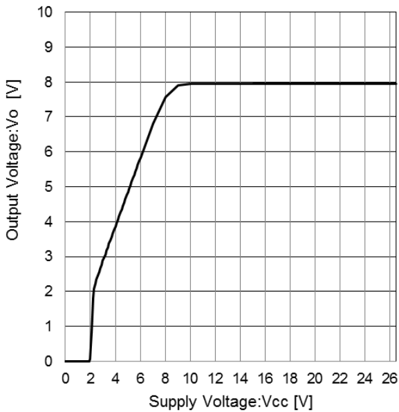
Figure 6. Line Regulation (Io=500mA)
