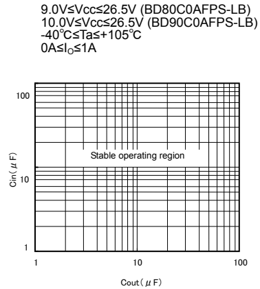
Cin vs Cout(reference data)
