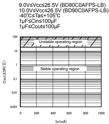
Cout_ESR vs Io(reference data)
