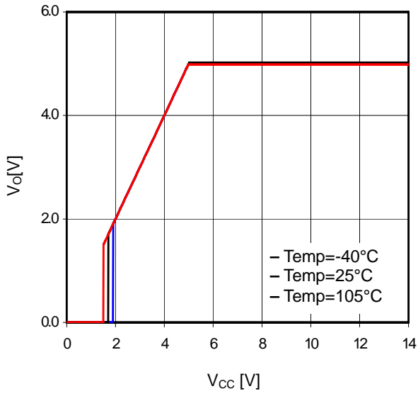
Figure 27. V_{CC}-V_o ( I_o=0mA )
