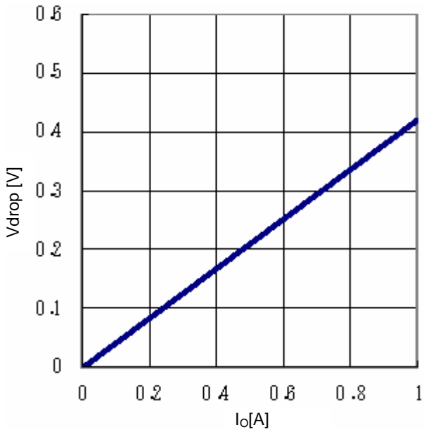
Fig.22 Minimum dropout Voltage 3 (V CC =6V、Ta=25°C)
