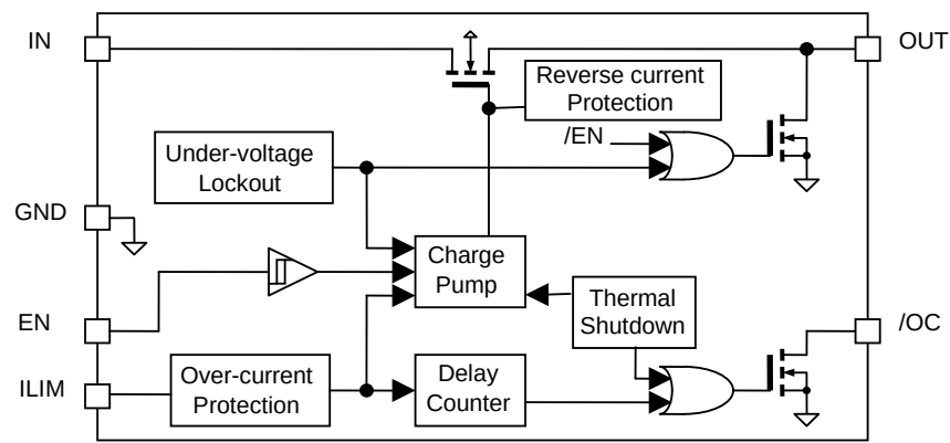
Figure 2. Block Diagram
