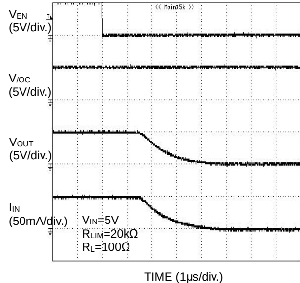
Figure 37. Output Fall Characteristic
