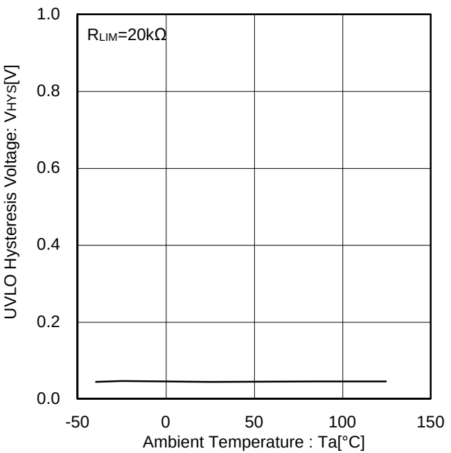
Figure 23. UVLO Hysteresis Voltage vs Ambient Temperature
