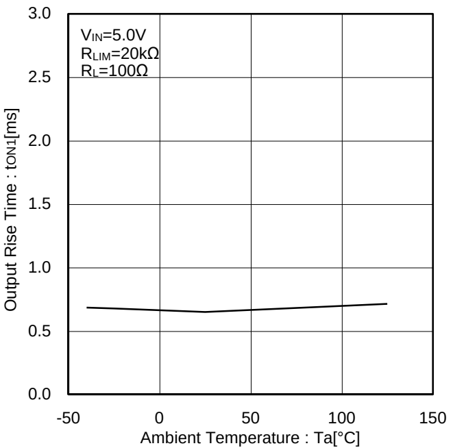
Figure 25. Output Rise Time vs Ambient Temperature
