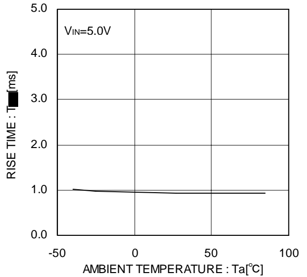
Figure 18. Output rise time
