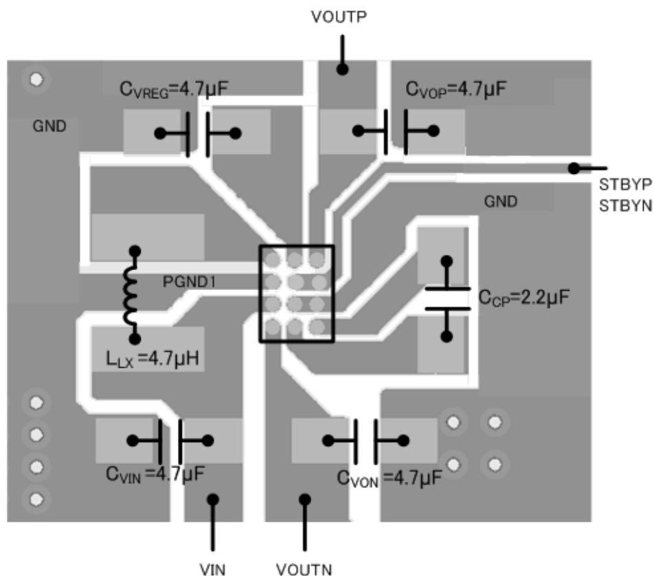
Figure 24. Suggested Layout
