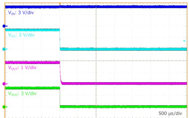
Figure 59. EN Shutdown at R_{Load} = 0.9\ \Omega ( V_{IN} = 5.0\text{ V} , V_{OUT} = 1.8\text{ V} , V_{EN} = 5\text{ V to }0\text{ V} )
