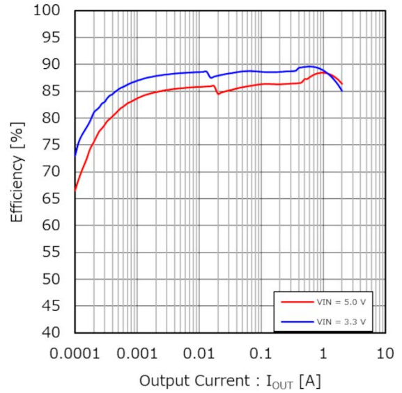
Figure 29. Efficiency vs Output Current (V OUT = 0.9 V)
