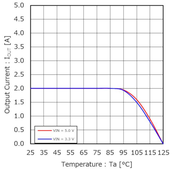
Figure 67. Thermal Derating ( V_{OUT} = 1.2\text{ V} )
