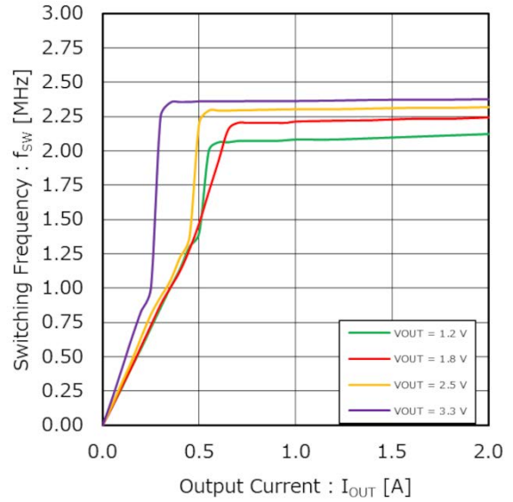
Figure 41. Switching Frequency vs Output Current (VIN = 5.0 V)
