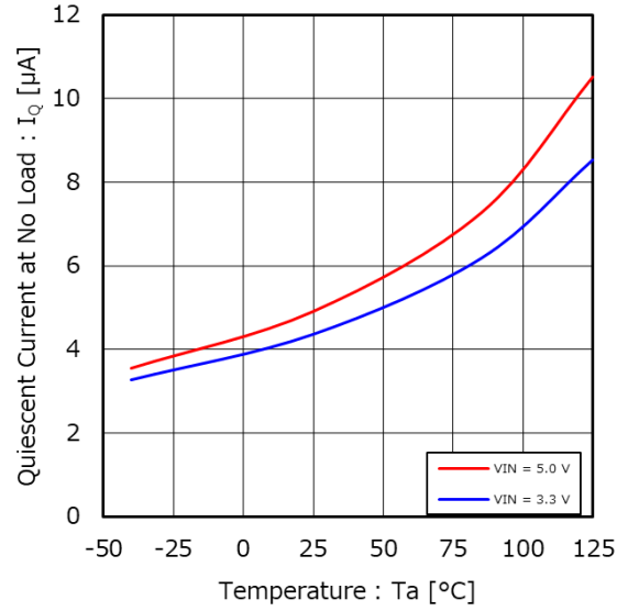
Figure 2. Quiescent Current at No Load vs Temperature
