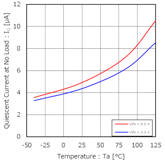
Figure 2. Quiescent Current at No Load vs Temperature
