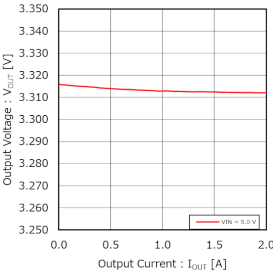
Figure 39. Output Voltage vs Output Current (Load Regulation) ( V_{OUT} = 3.3\text{ V} )
