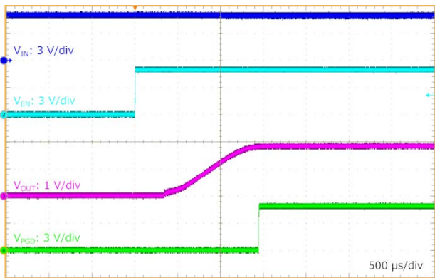
Figure 58. EN Start-up at RLoad = 0.9 Ω (VIN = 5.0 V, VOUT = 1.8 V, VEN = 0 V to 5 V)
