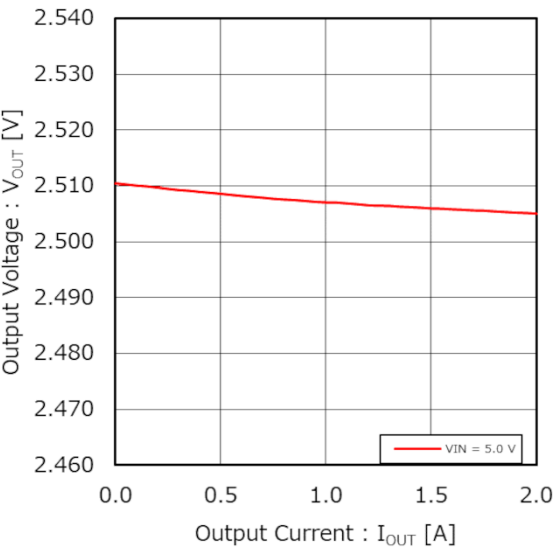
Figure 38. Output Voltage vs Output Current (Load Regulation) ( V_{OUT} = 2.5\text{ V} )
