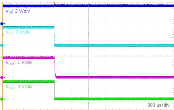
Figure 59. EN Shutdown at RLoad = 0.9 Ω (VIN = 5.0 V, VOUT = 1.8 V, VEN = 5 V to 0 V)
