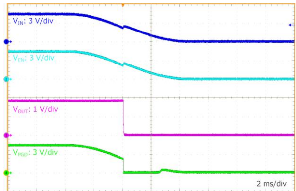
Figure 63. VIN Shutdown at R_{Load} = 0.9\ \Omega ( V_{IN} = V_{EN} = 5\text{ V} to 0\text{ V} , V_{OUT} = 1.8\text{ V} )
