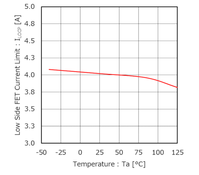
Figure 13. Low Side FET Current Limit vs Temperature
