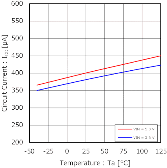
Figure 2. Circuit Current vs Temperature
