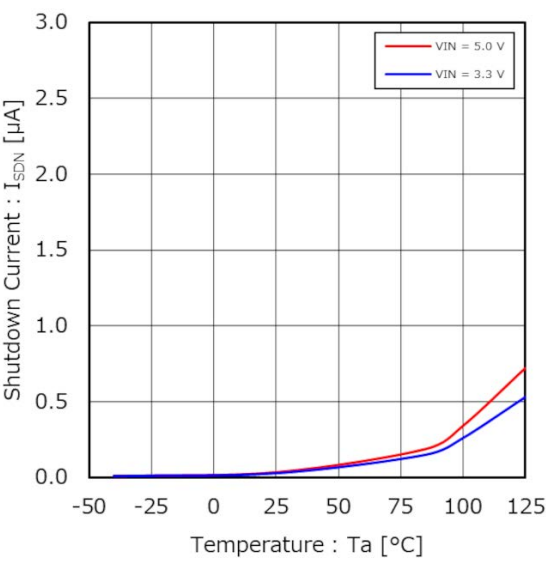
Figure 1. Shutdown Current vs Temperature
