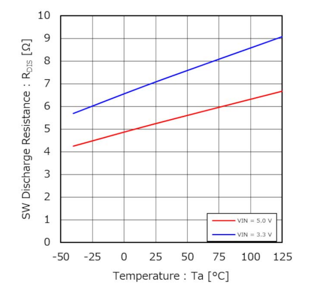
Figure 14. SW Discharge Resistance vs Temperature
