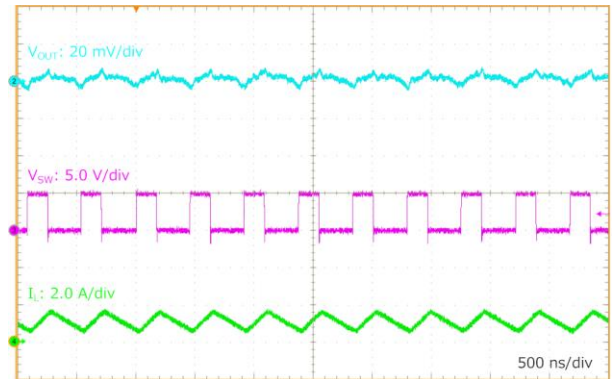
Figure 49. Output Ripple Voltage ( V_{IN} = 5.0 V, V_{OUT} = 1.8 V, I_{OUT} = 1.0 A)
