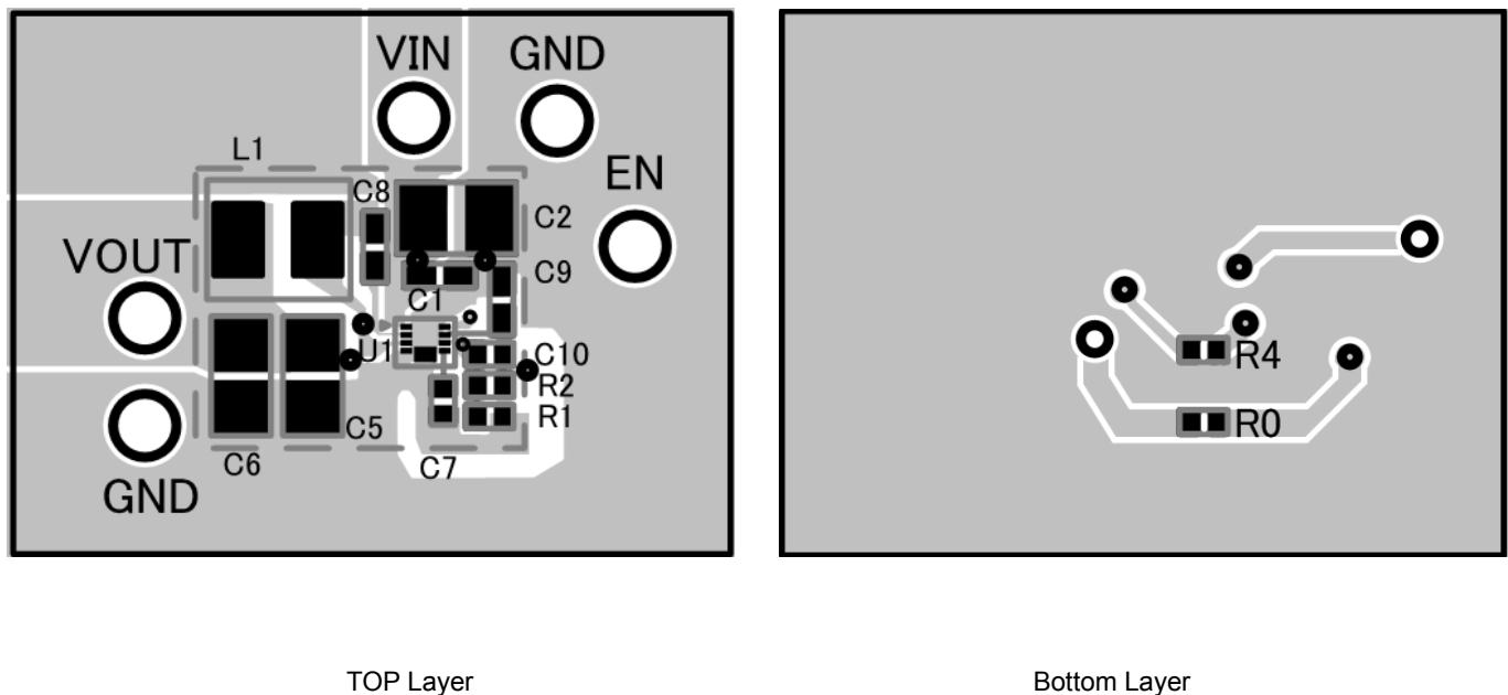
Figure 63. Example of PCB layout
