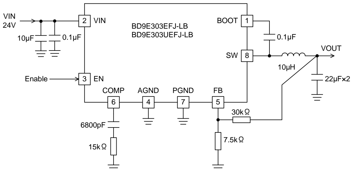
Figure 1. Application circuit
