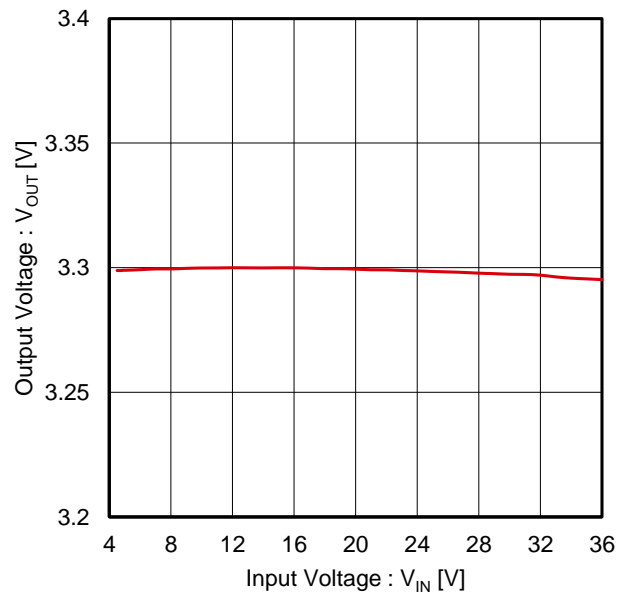
Figure 52. Line Regulation (VOUT = 3.3 V, IOUT = 2 A, 600 kHz_IOUTMAX = 5 A_PWM setting)
