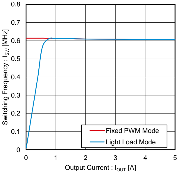
Figure 49. Switching Frequency vs Output Current (VIN = 12 V, VOUT = 3.3 V, 600 kHz_IOUTMAX = 5 A setting)
