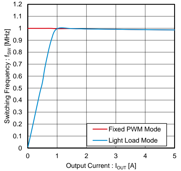
Figure 50. Switching Frequency vs Output Current (VIN = 12 V, VOUT = 3.3 V, 1 MHz_IOUTMAX = 5 A setting)
