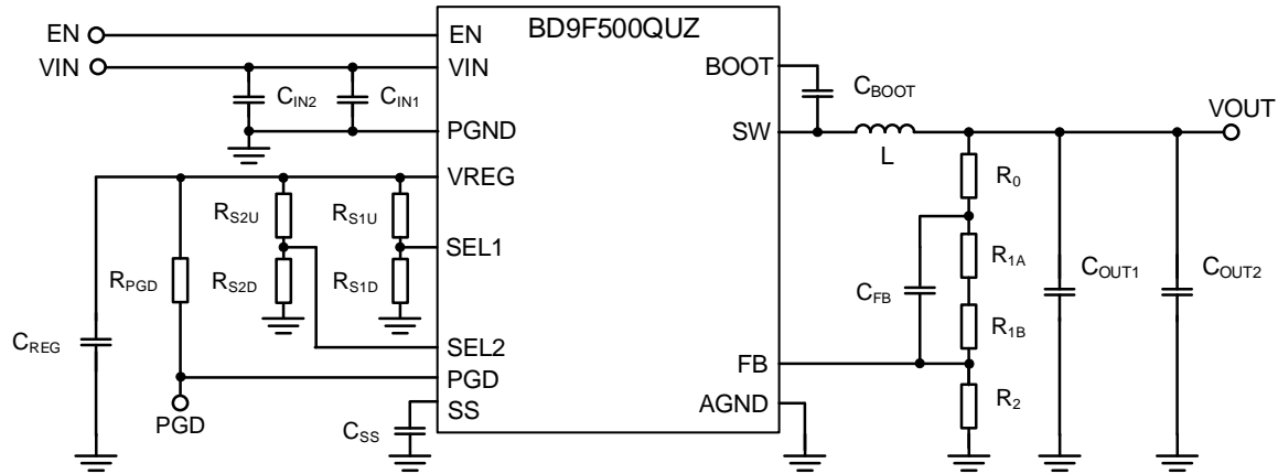
Figure 87. Application Circuit
