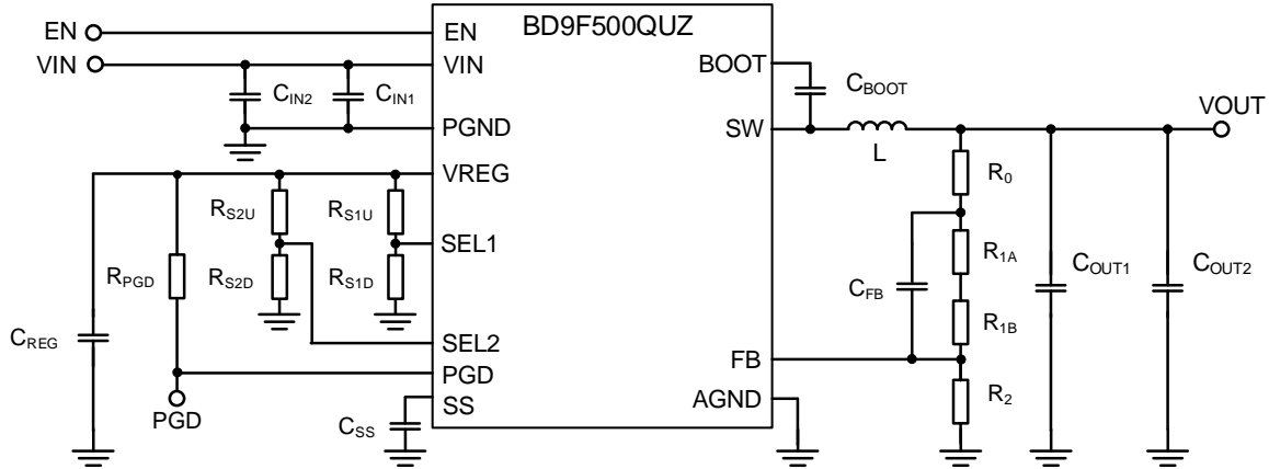
Figure 97. Application Circuit
