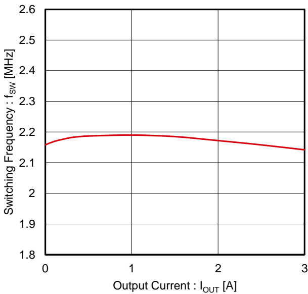
Figure 51. Switching Frequency vs Output Current (VIN = 12 V, VOUT = 3.3 V, 2.2 MHz setting)
