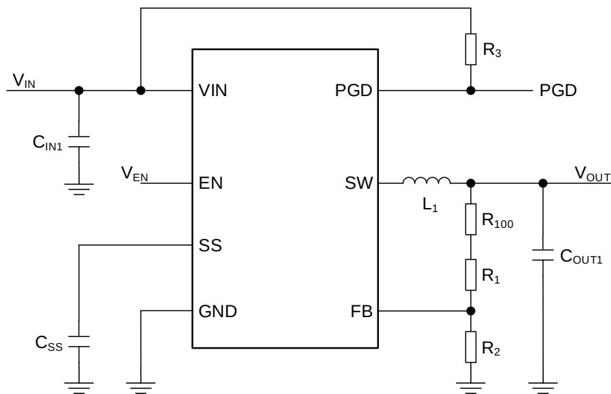
Figure 24. Typical Application
