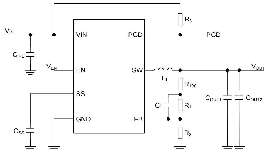
Figure 29. Reference Circuit 1
