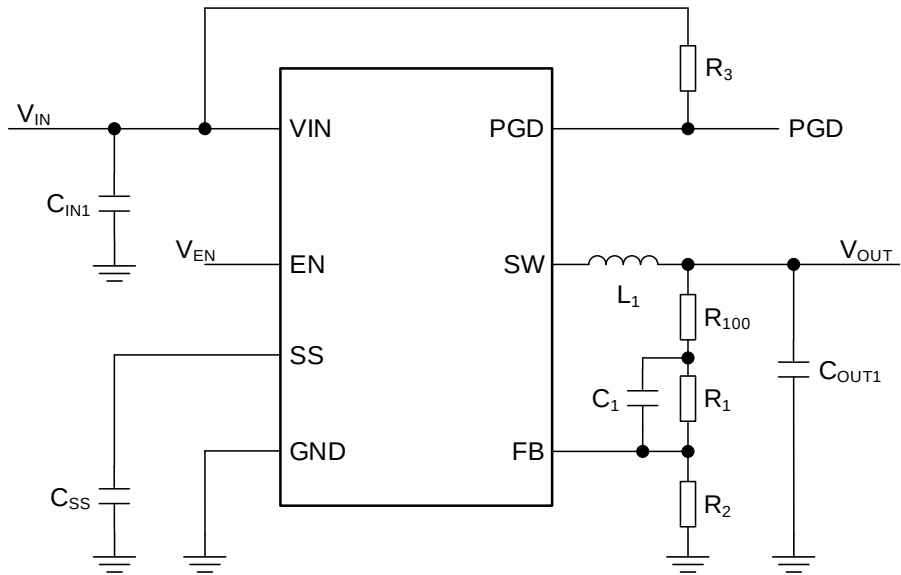
Figure 49. Reference Circuit 5
