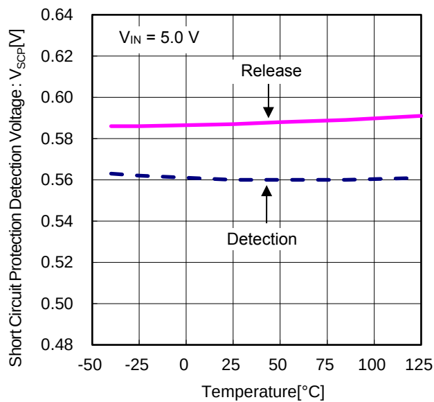
Figure 17. Short Circuit Protection Detection Voltage
