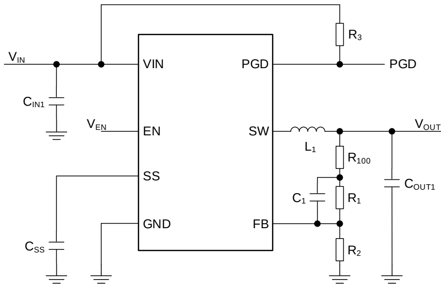
Figure 45. Reference Circuit 4
