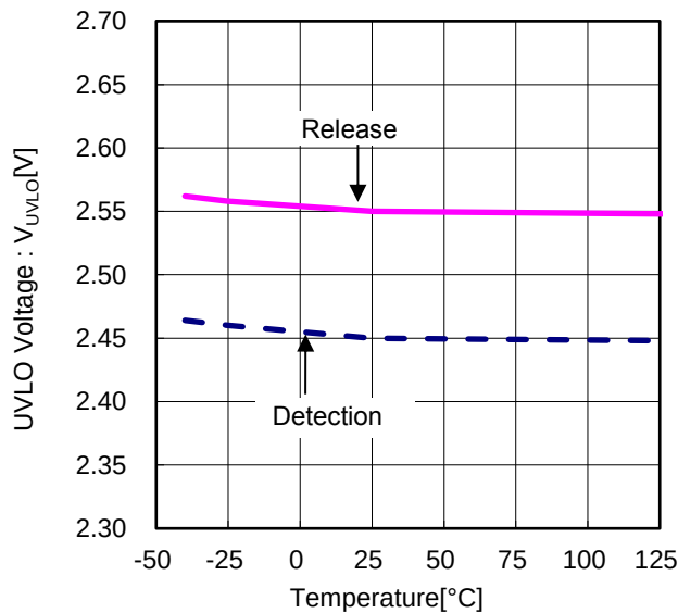
Figure 13. UVLO Detection Voltage vs Temperature
