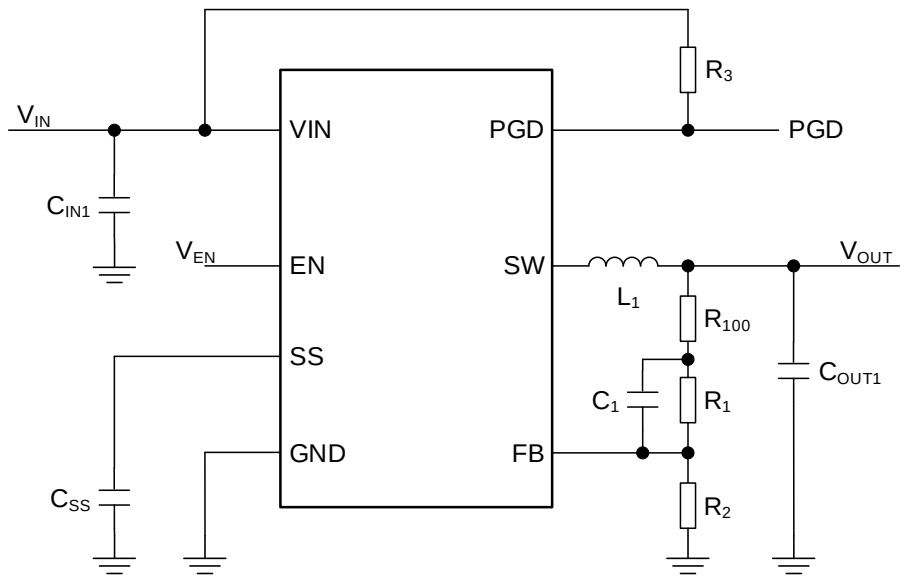
Figure 50. Reference Circuit 5
