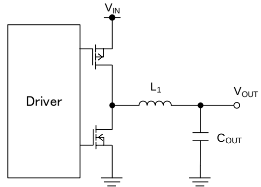
Figure 28. Output LC Filter Circuit
