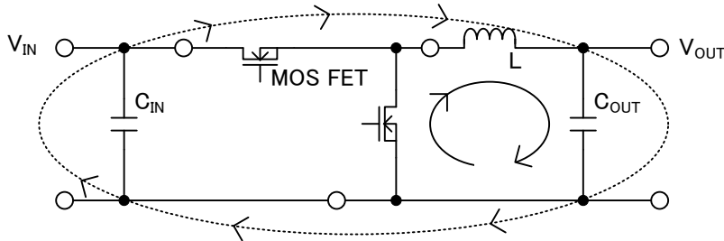
Figure 53. Current Loop of Buck DC/DC Converter
