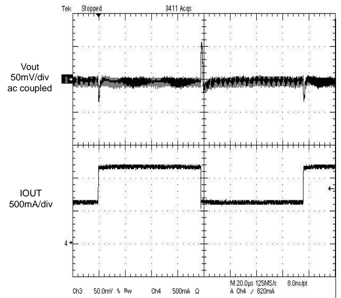
Figure 8. Load transient response 600mA to 1200mA tr=tf=100ns, MODE : Low
