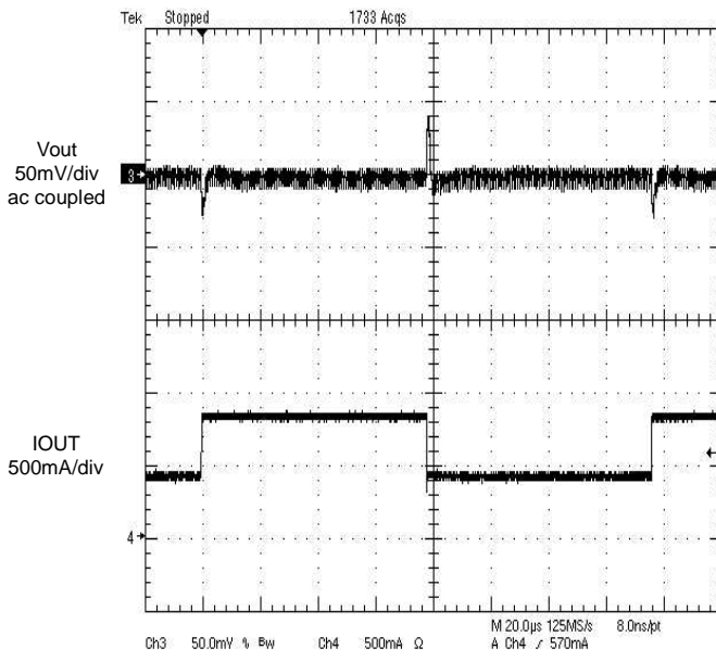
Figure 7. Load transient response 400mA to 800mA tr=tf=100ns, MODE : Low
