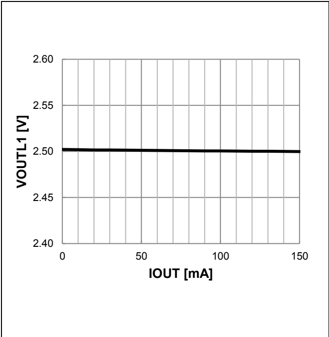
Figure 50. VOUTL1 Output Voltage vs IOU
