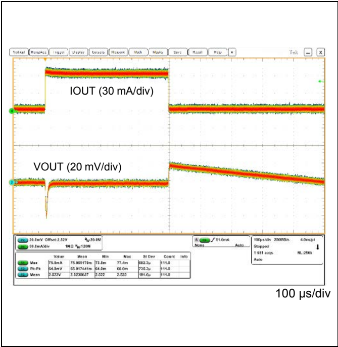
Figure 75. VOUTL1 Load Transient (IOUT = 0 A to 75 mA (SR = 100 mA/μs))
