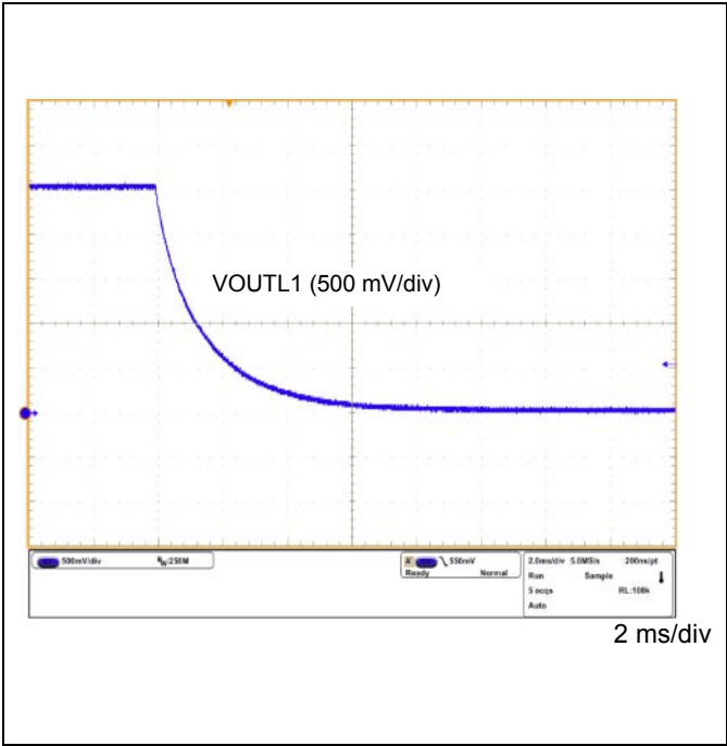
Figure 68. VOUTL1 Power OFF Waveform
