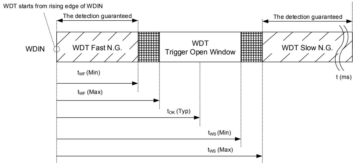
Figure 34. WDT Function
