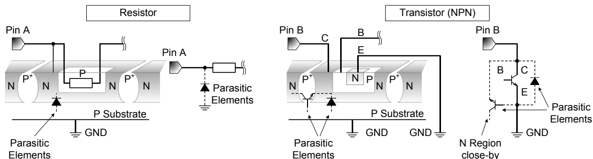
Figure 76. Example of Monolithic IC Structure
