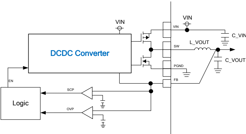
Figure 31. Power Abnormality Monitoring Circuit
