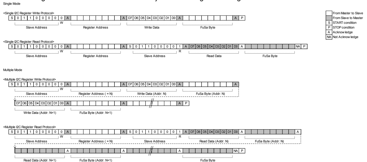
Figure 24. I2C Protocol (FuSa Mode)
