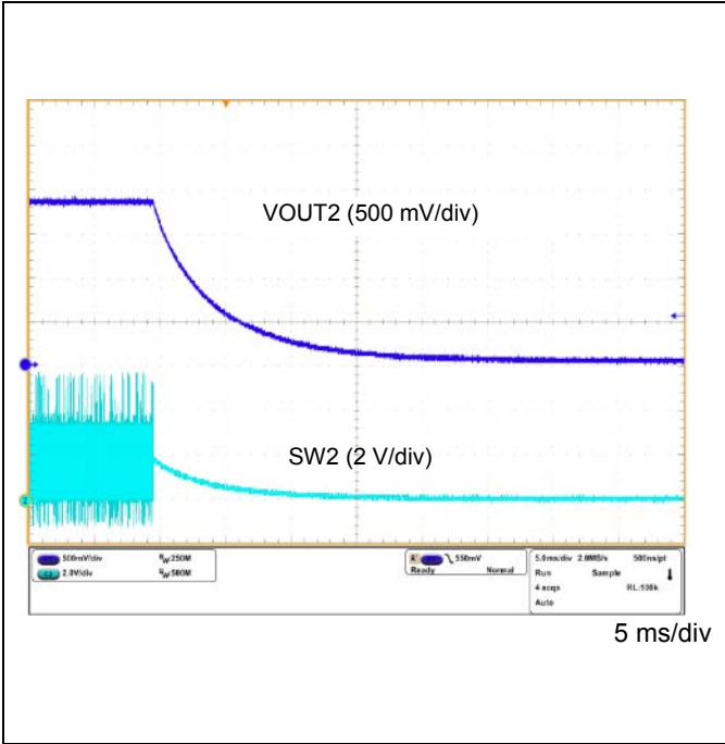
Figure 64. VOUT2 Power OFF Waveform
