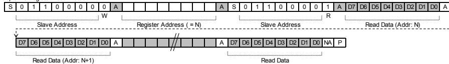
Figure 23. I2C Protocol (Each Access Mode)
