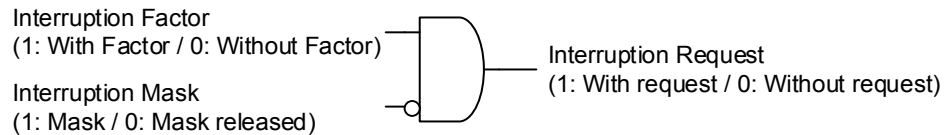
Figure 28. Interruption Factor/Mask/Request
