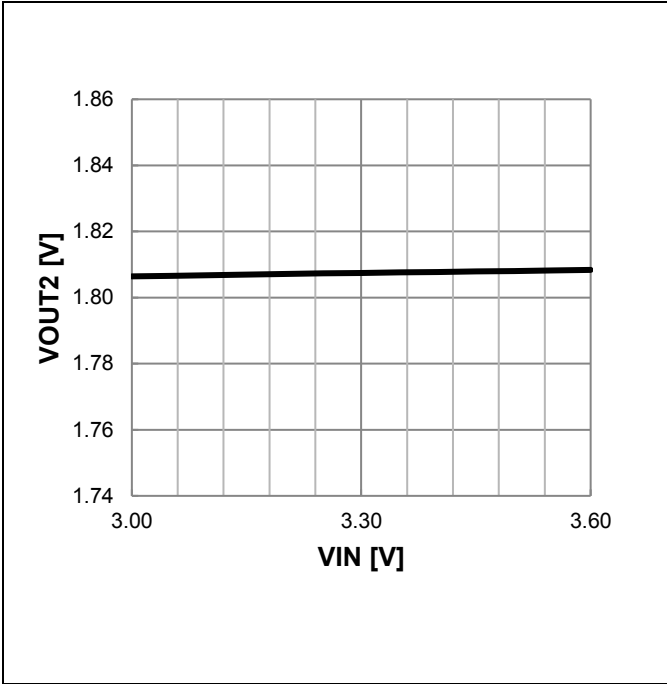
Figure 40. VOUT2 Output Voltage vs VIN
