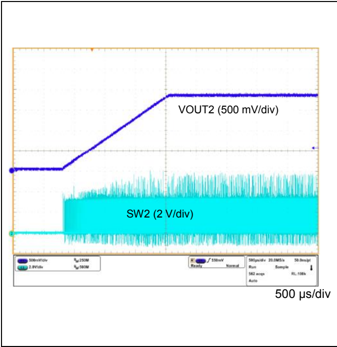
Figure 57. VOUT2 Power ON Waveform
