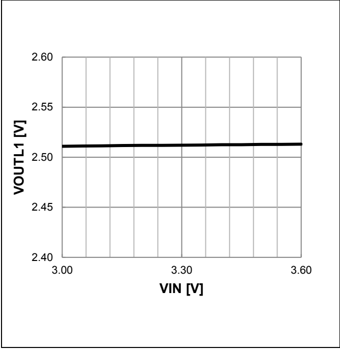
Figure 44. VOUTL1 Output Voltage vs VIN
