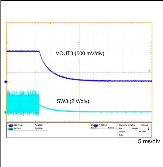
Figure 66. VOUT3 Power OFF Waveform (VOUT3 = 1.5 V Setting)
