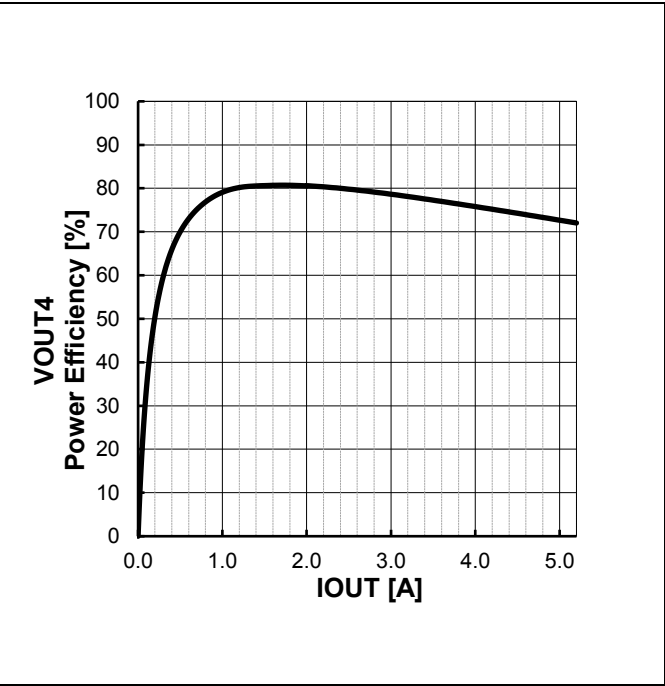
Figure 55. VOUT4 Power Efficiency vs IOU T
