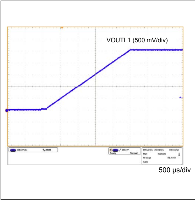
Figure 61. VOUTL1 Power ON Waveform
