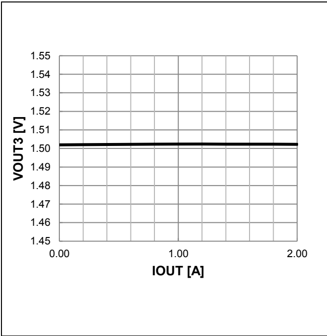
Figure 48. VOUT3 Output Voltage vs IOU (VOUT3 = 1.5 V Setting)
