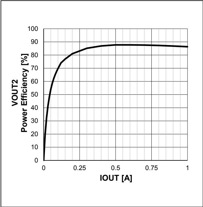
Figure 52. VOUT2 Power Efficiency vs IOUT
