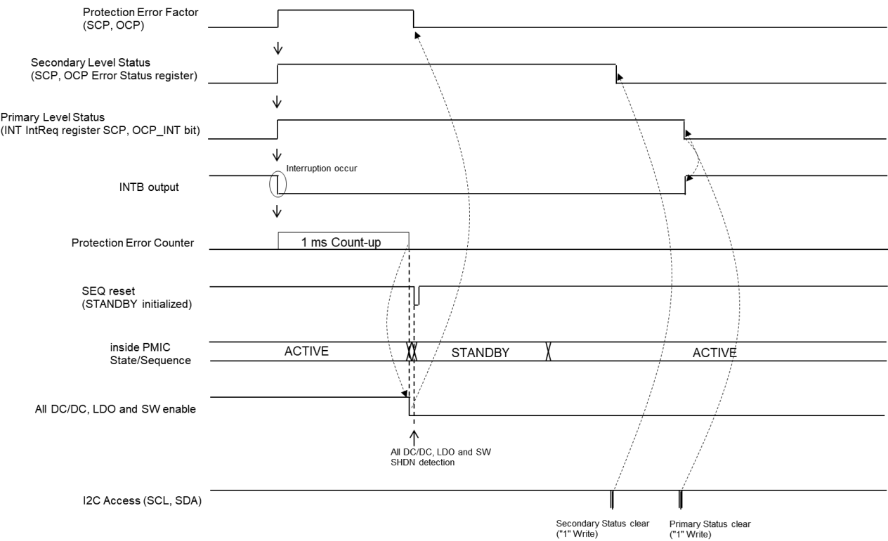
Figure 32. Timing Chart when Protection Error Factor Occur 1
