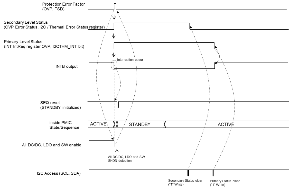
Figure 33. Timing Chart when Protection Error Factor Occur 2
