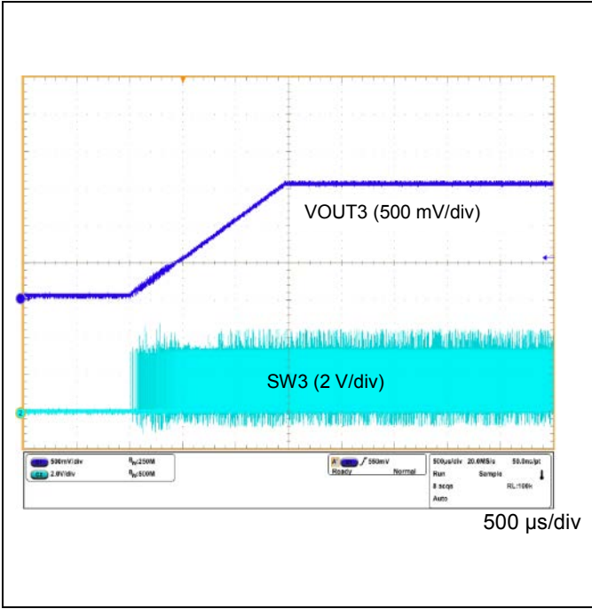
Figure 59. VOUT3 Power ON Waveform (VOUT3 = 1.5 V Setting)
