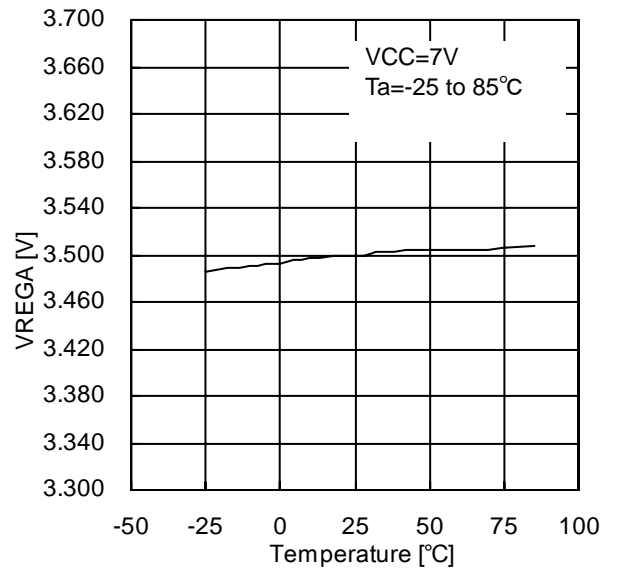
Figure.15 VREGA – Ta
