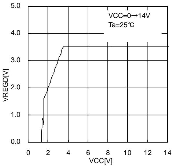
Figure.16 VREGD- VCC
