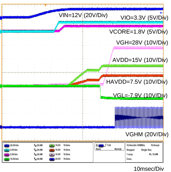
Figure 8. Power-on 2 (VGL driven AVDD switch node)
