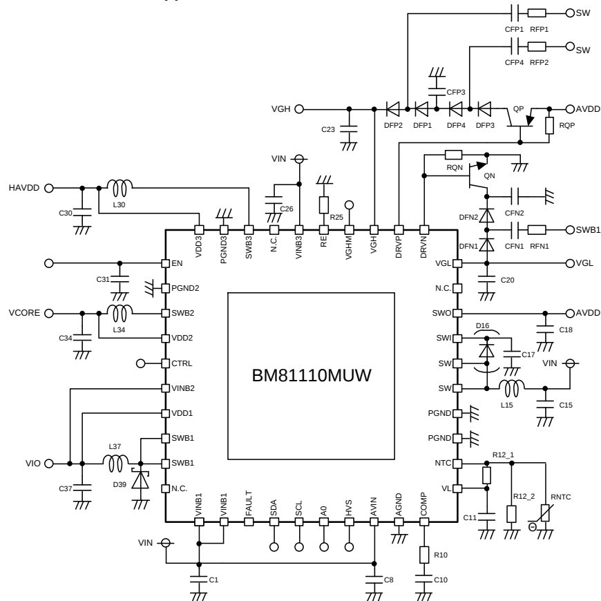
Figure 41. Example Application
