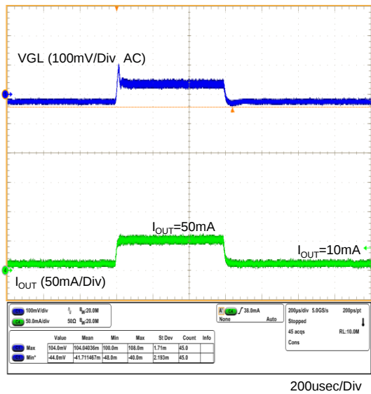
Figure 33. VGL Load Transient
