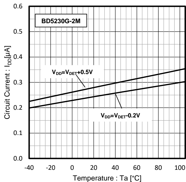
Figure 8. Circuit Current vs. Temp
