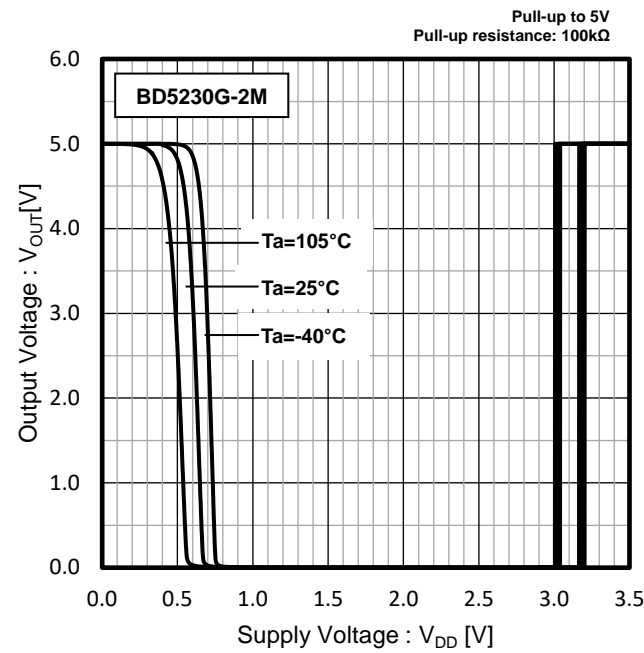
Figure 17. I/O Characteristics
