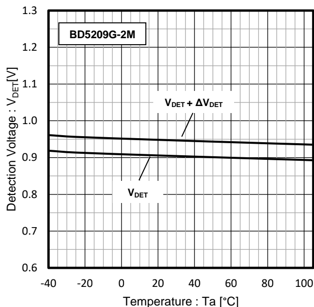
Figure 12. Detection Voltage and Release Voltage
