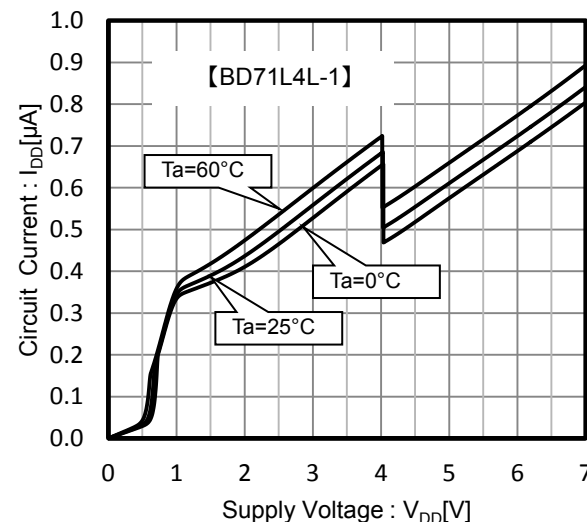
Figure 3. Circuit Current
